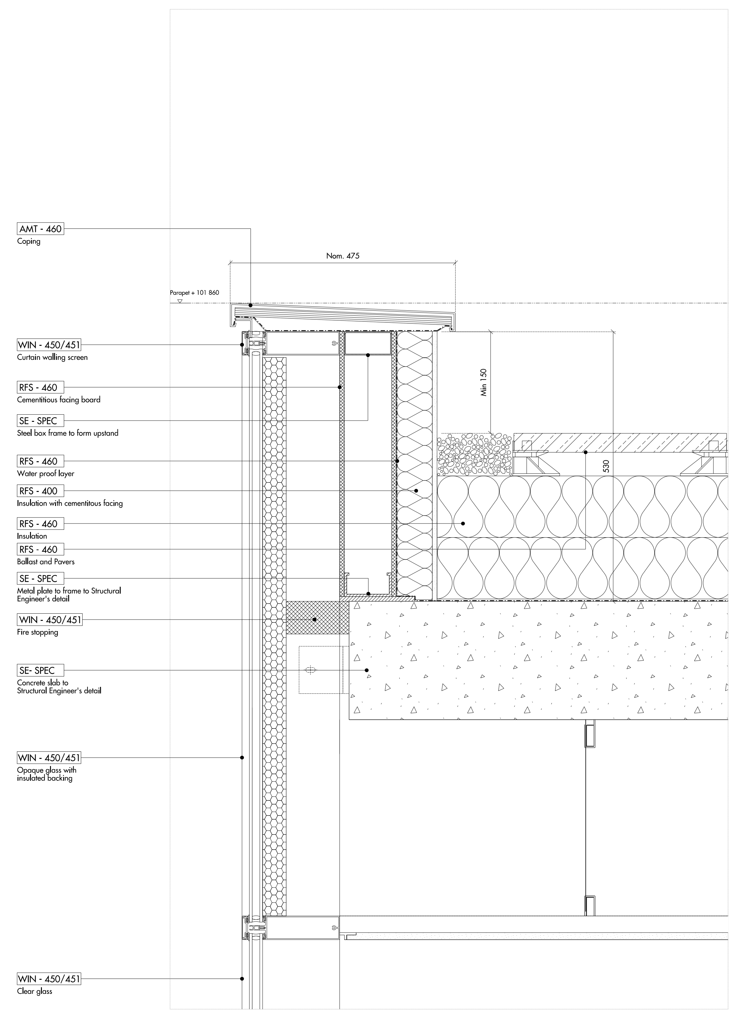
02 DETAIL SECTION
