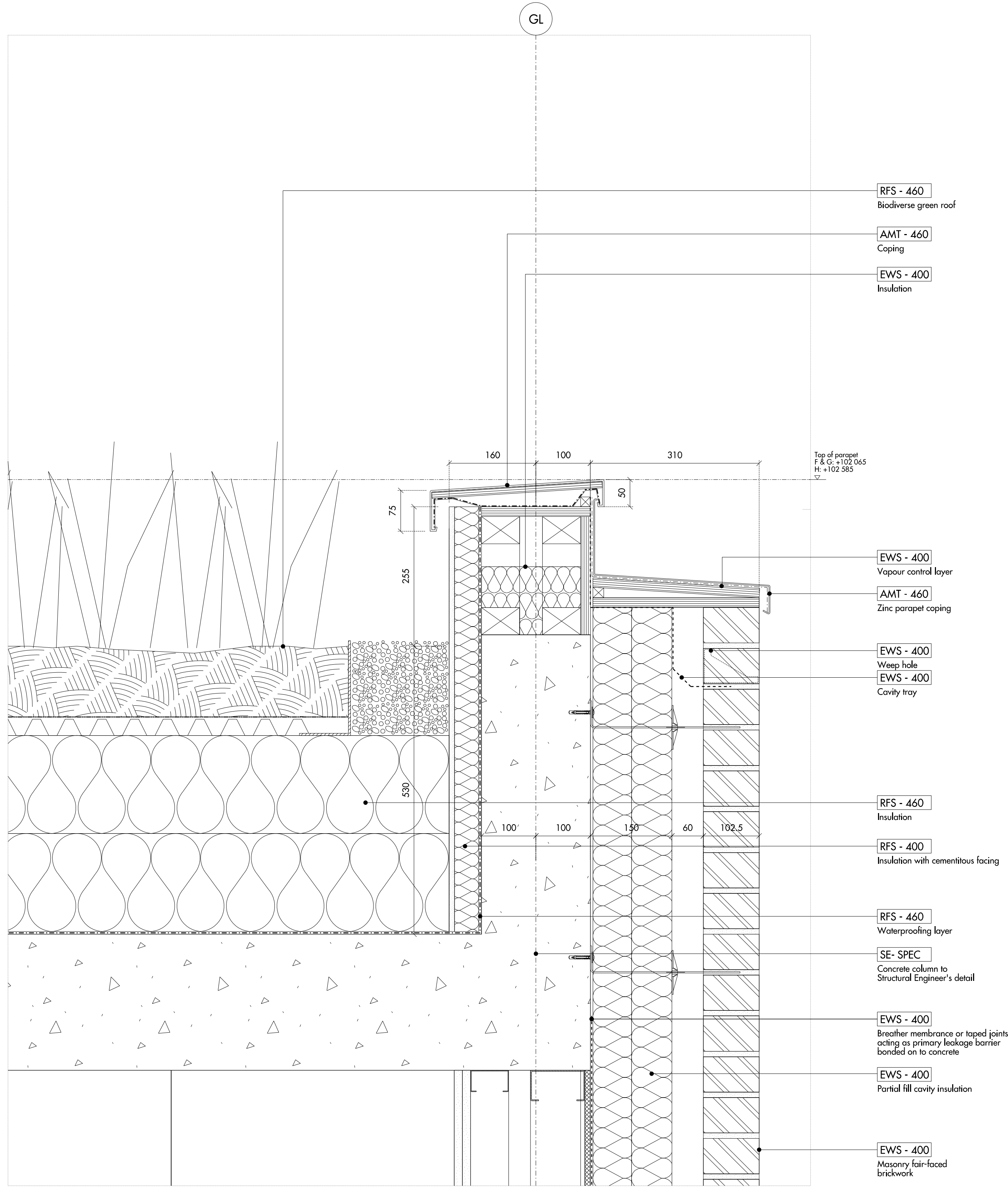
01 DETAIL SECTION
