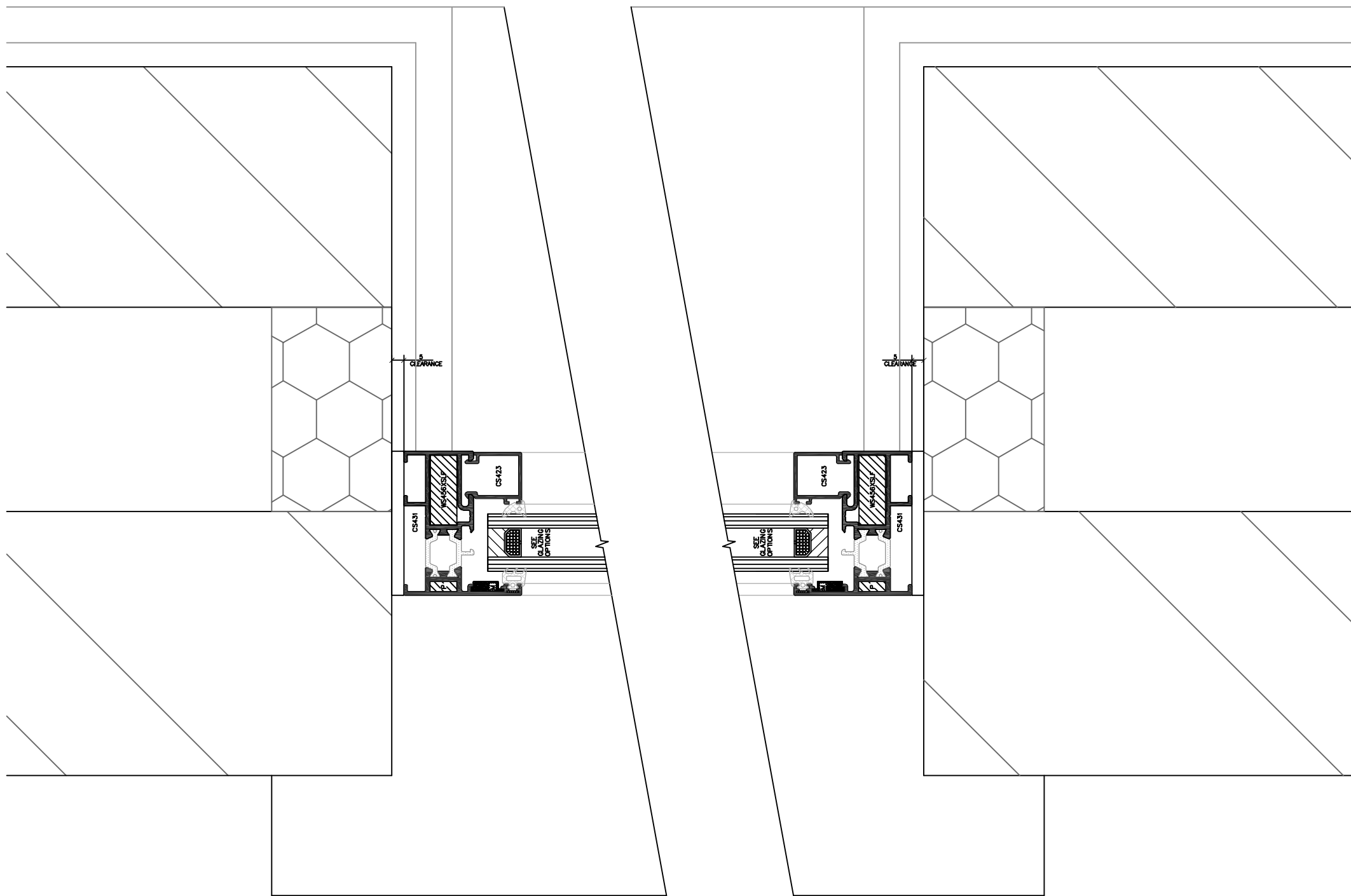
SECTION Z-Z
