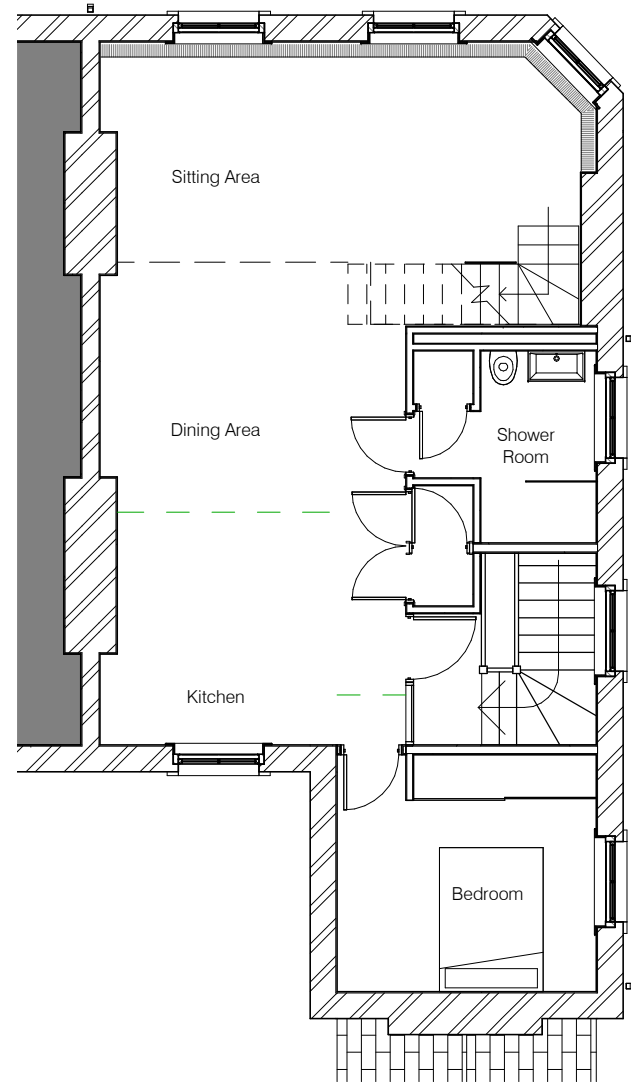
Proposed Third Floor Plan
