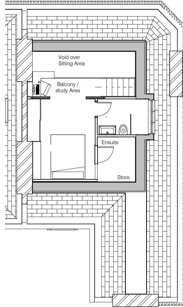
Proposed Mezzanine / Attic plan
