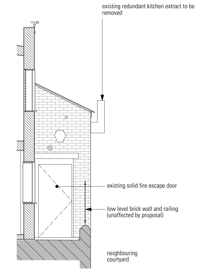
Ex04 Existing Elevation 04 Scale 1:50@A1, 1:100@A3
