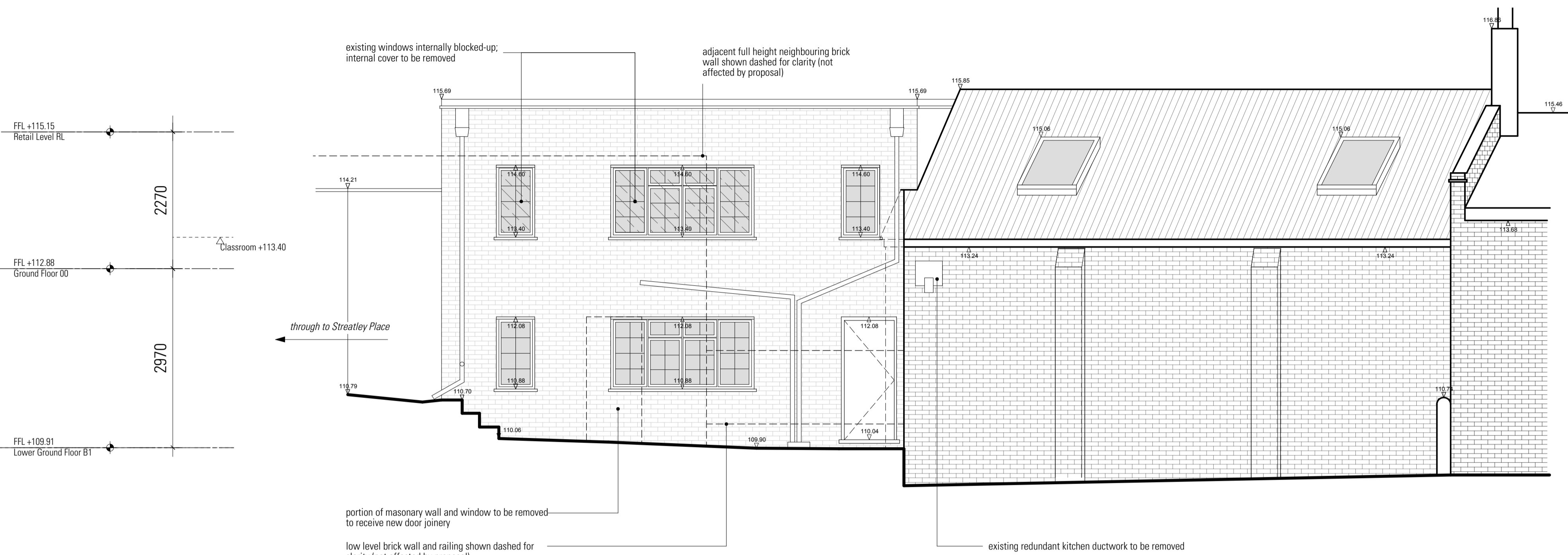
Ex03 Existing Elevation 03 Scale 1:50@A1, 1:100@A3
