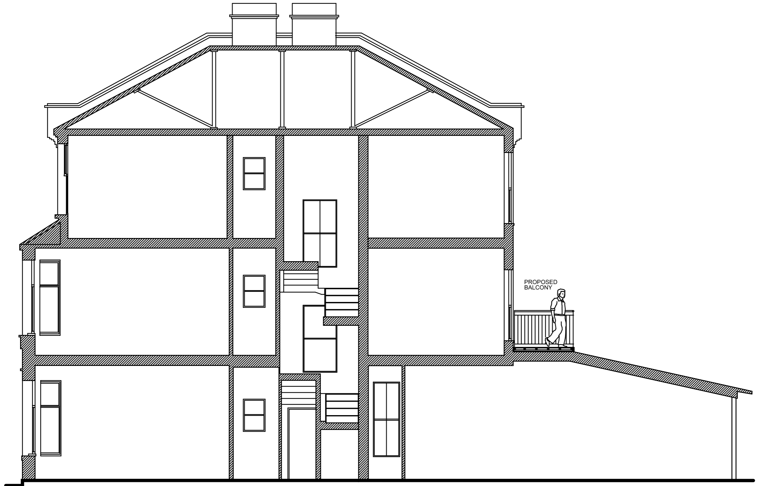
PROPOSED SECTION L/06
