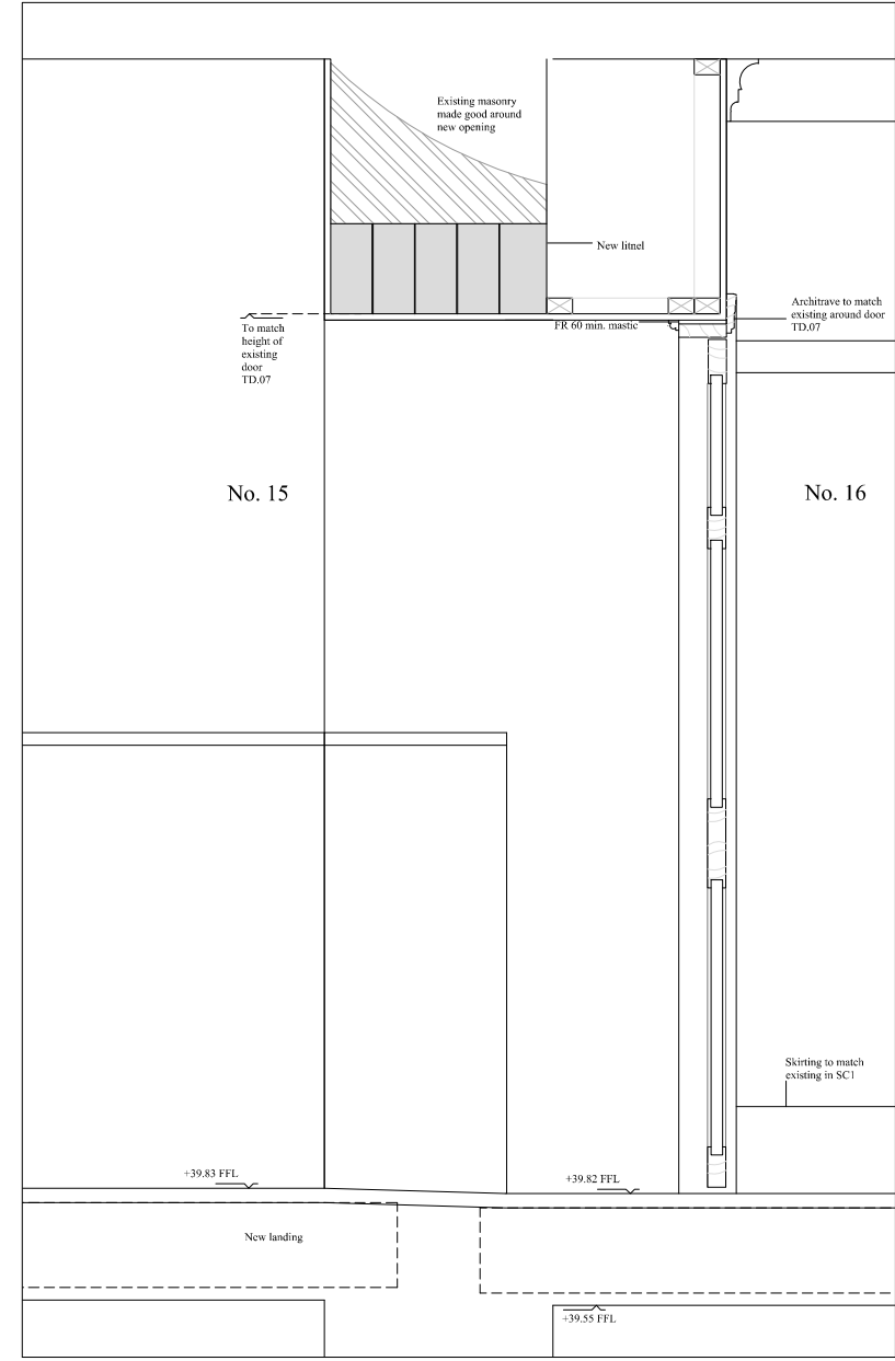
Proposed Section B
