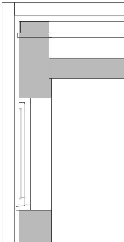
EXISTING CASEMENT WINDOW : SECTION SINGLE GLAZED
