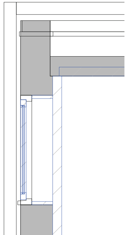
EXISTING CASEMENT WINDOW : SECTION DOUBLE GLAZED
