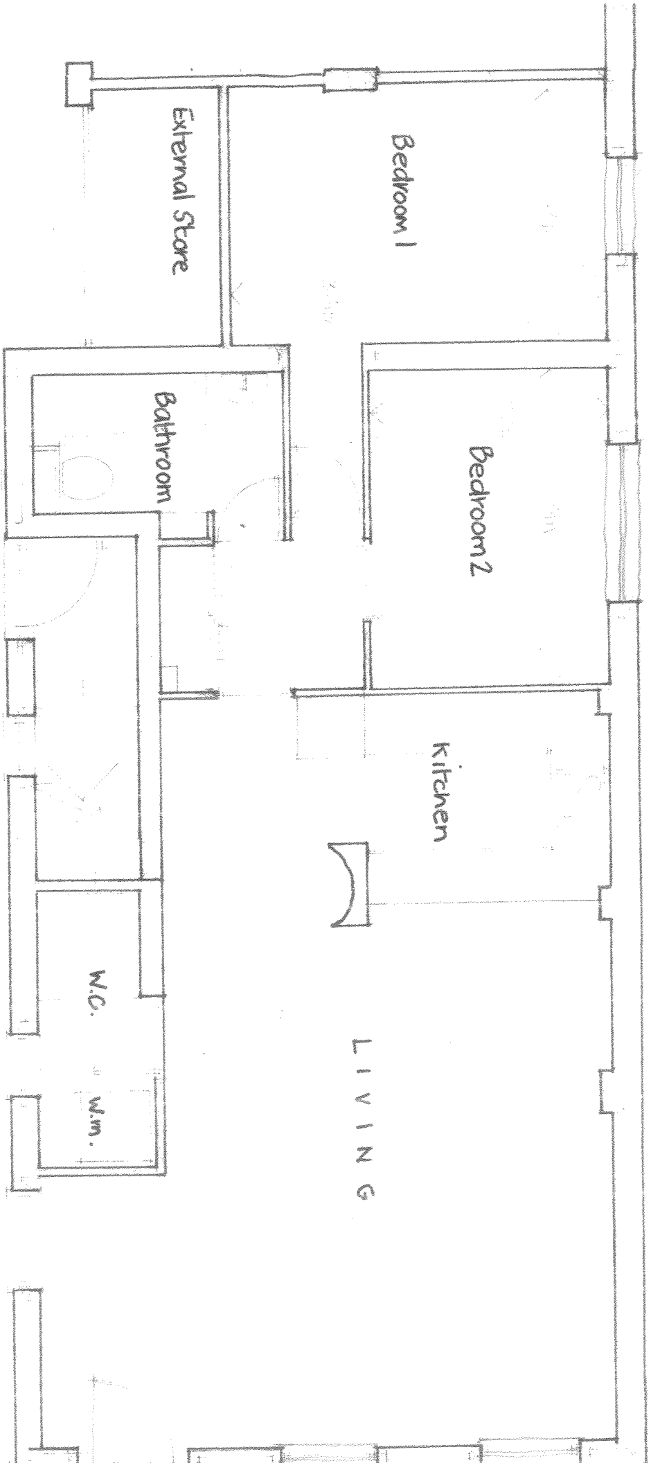
GROUND FLOOR FLAT 1A NETTLEY ST N.W.1 SCALE 1:50 FLOOR AREA 56.50 SQ.M.
