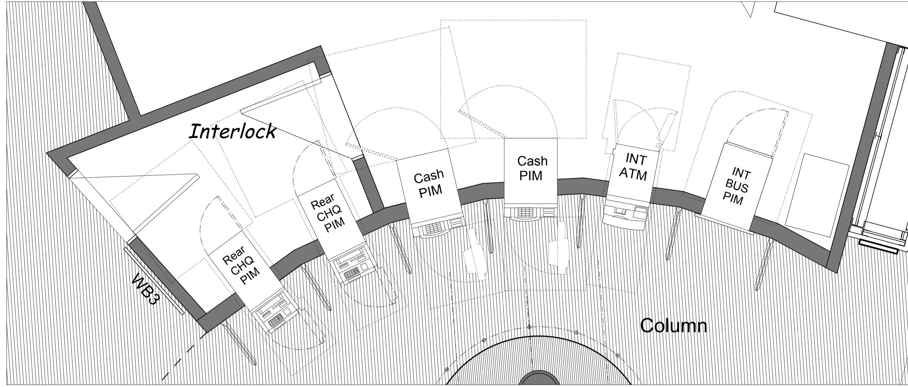
CAMDEN TOWN DETAILED PLAN OF AFFECTED AREA (scale 1:25) @ A1
