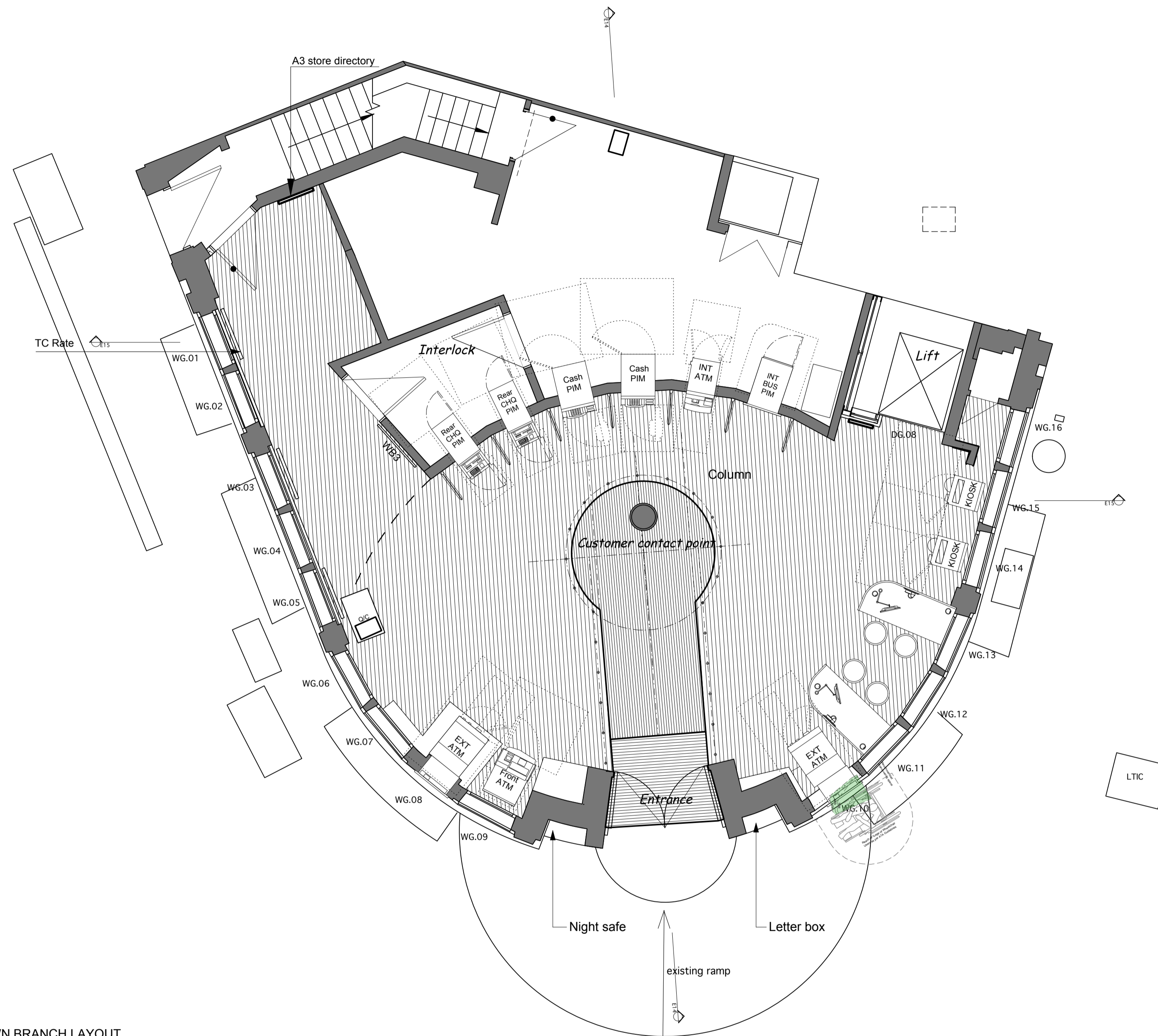
CAMDEN TOWN BRANCH LAYOUT INCLUDING REMOVAL & DELIVERY ROUTE (scale 1:50 @ A1)
