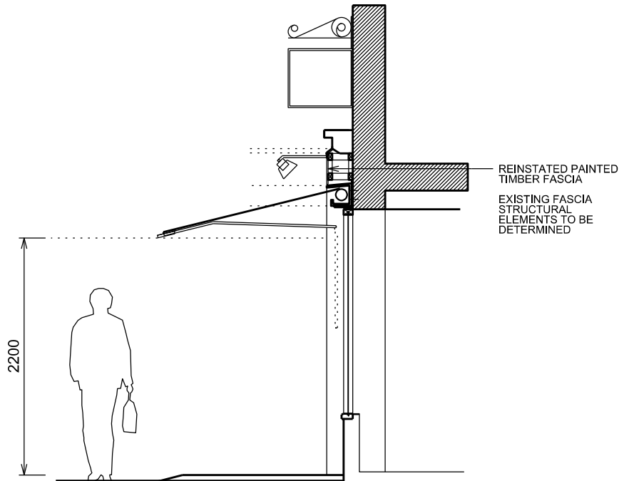
PROPOSED SECTION A-A - OPEN AWNING
