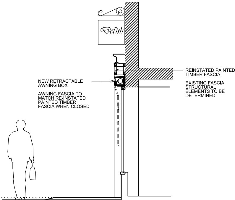
PROPOSED SECTION A-A - CLOSED AWNING
