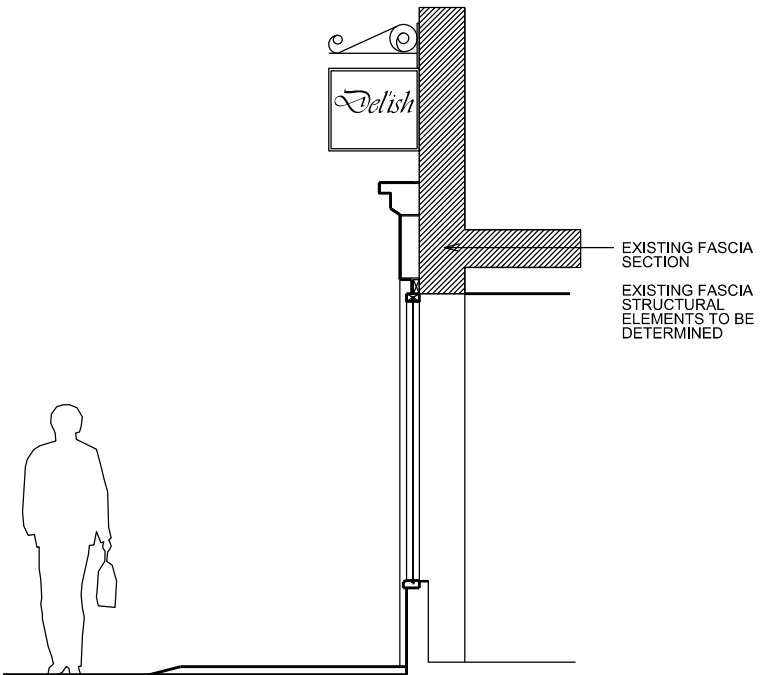
EXISTING SECTION OF FASCIA
