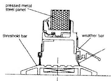
DOOR THRESHOLD
