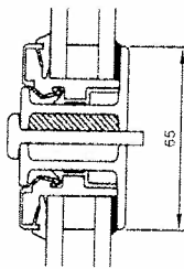
FIXED LIGHT/FIXED LIGHT COUPLING
