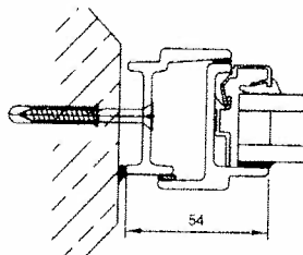
SHORT LEG OPENING CASEMENT JAMB
