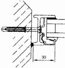
SHORT LEG FIXED LIGHT JAMB (EXTERNALLY GLAZED)
