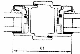
FRENCH CASEMENT CENTRAL STYLE
