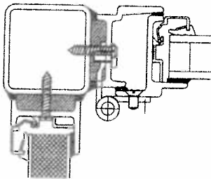
CORNER DETAIL
