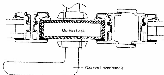
DOOR LOCK PANEL/MEETING STYLE
