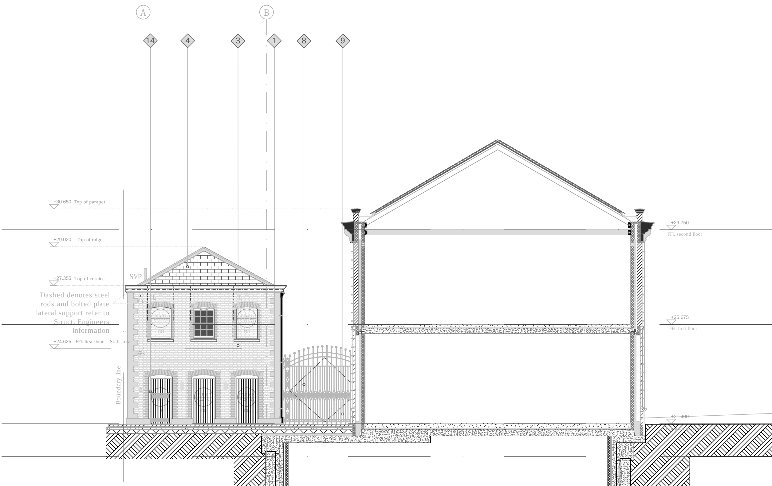
SOUTH WEST COURTYARD ELEVATION
