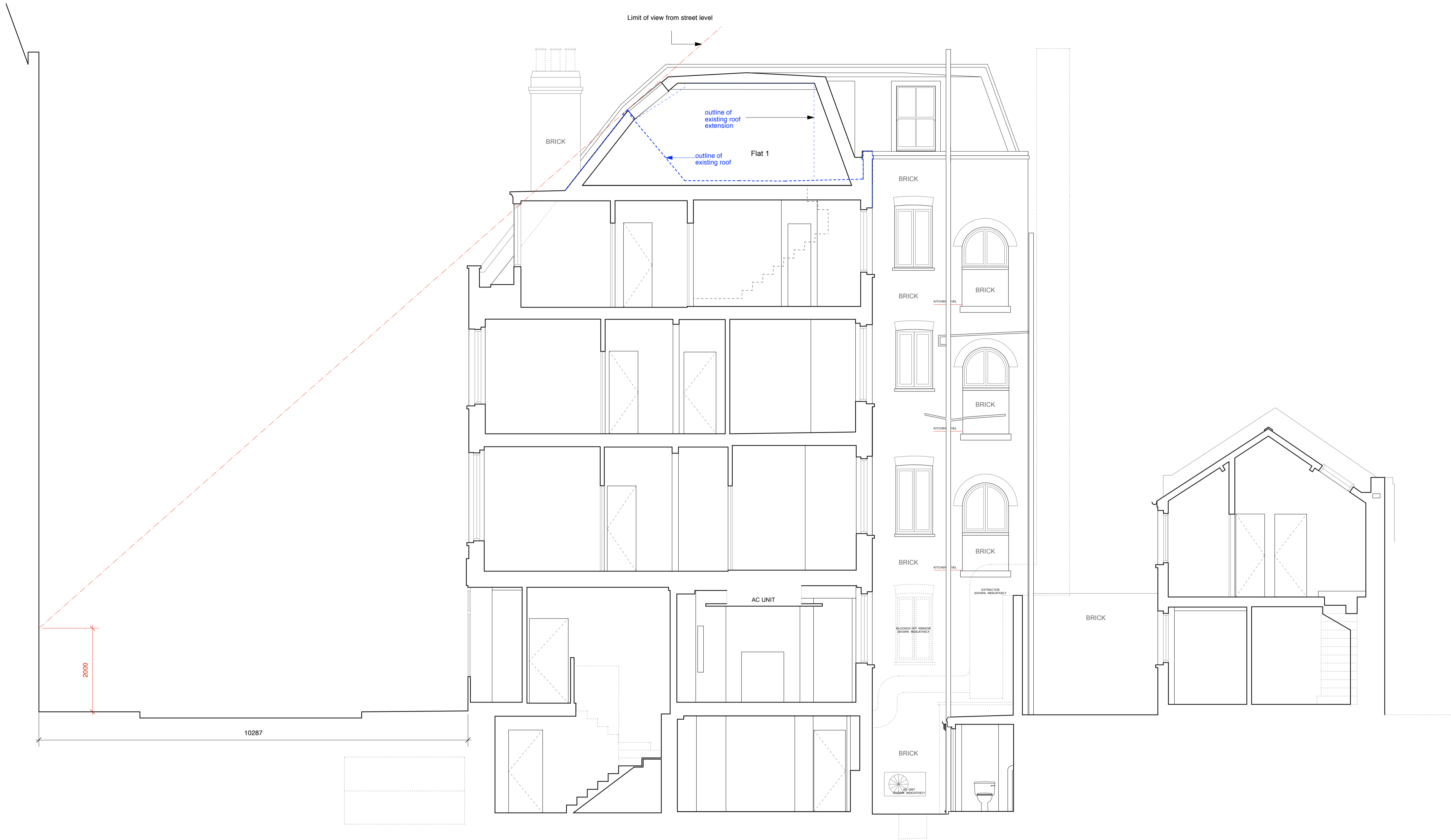
01/P13 Proposed Section
