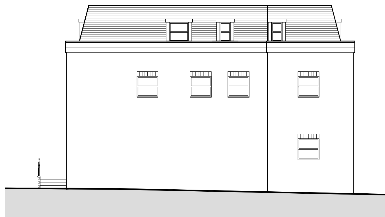
East Elevation
