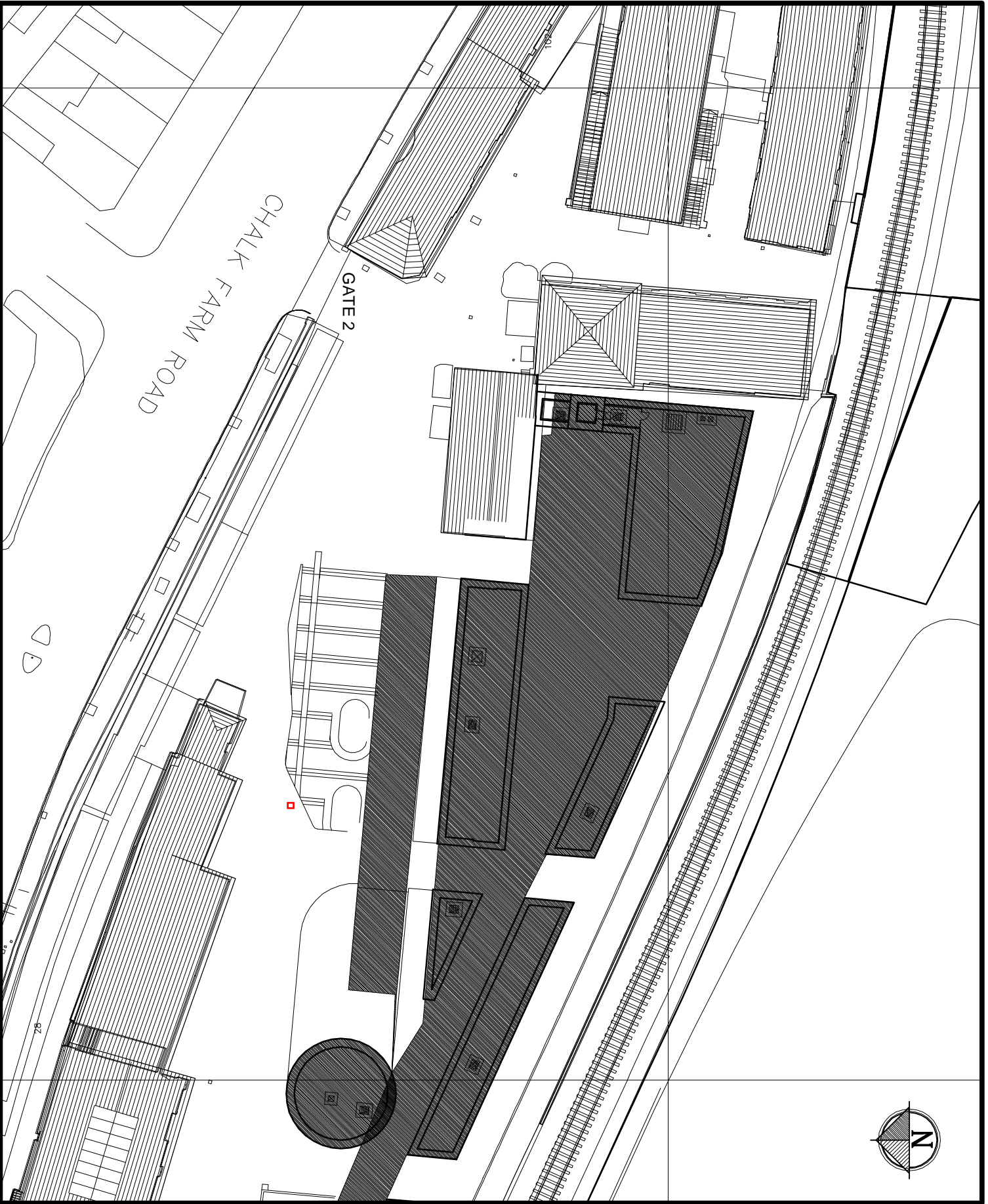
Stables Market Camden Site Plan Location for Bronze statue Scale 1:500 @ A4
