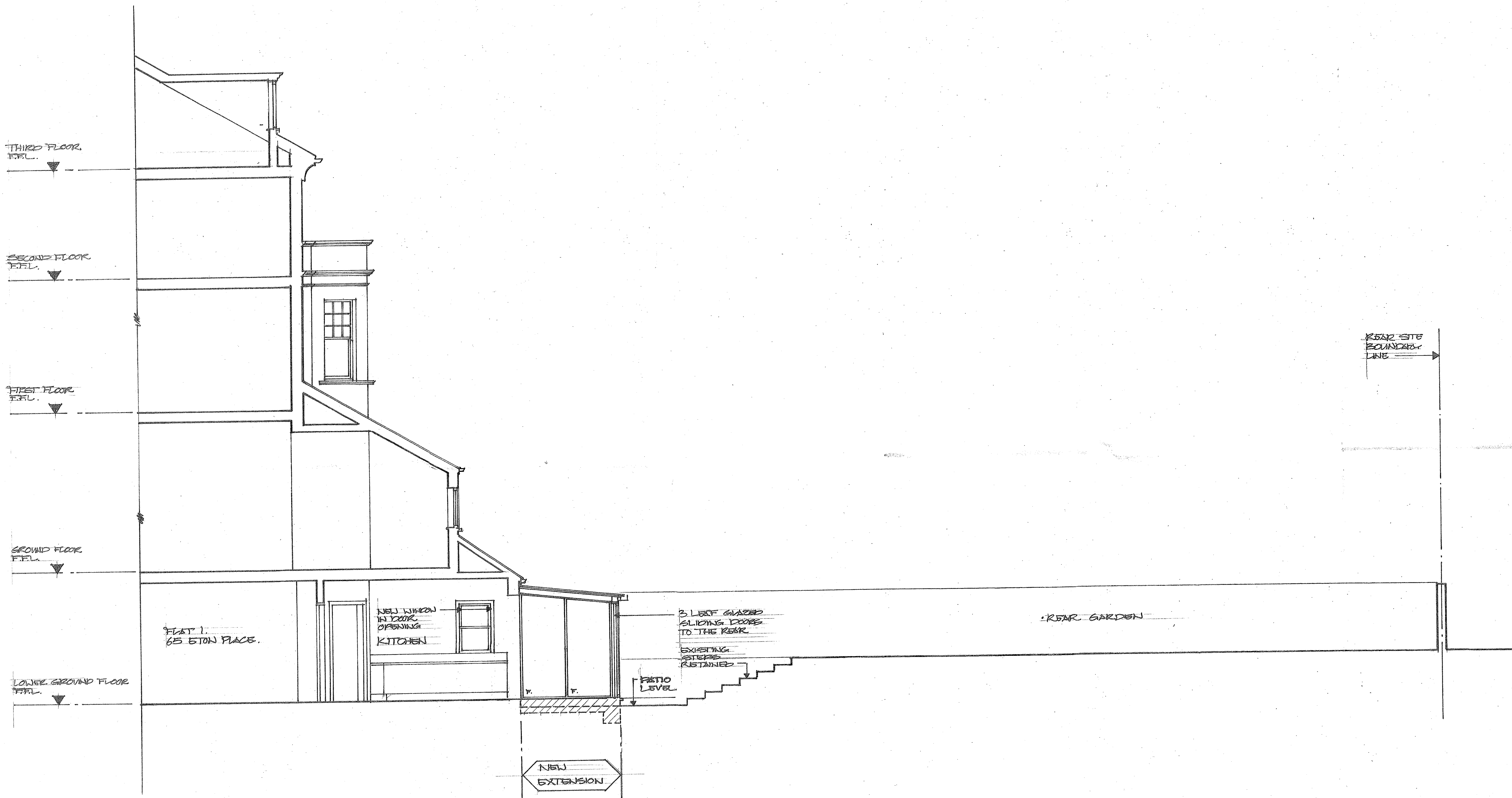
PROPOSED SECTION \frac{B}{10}
