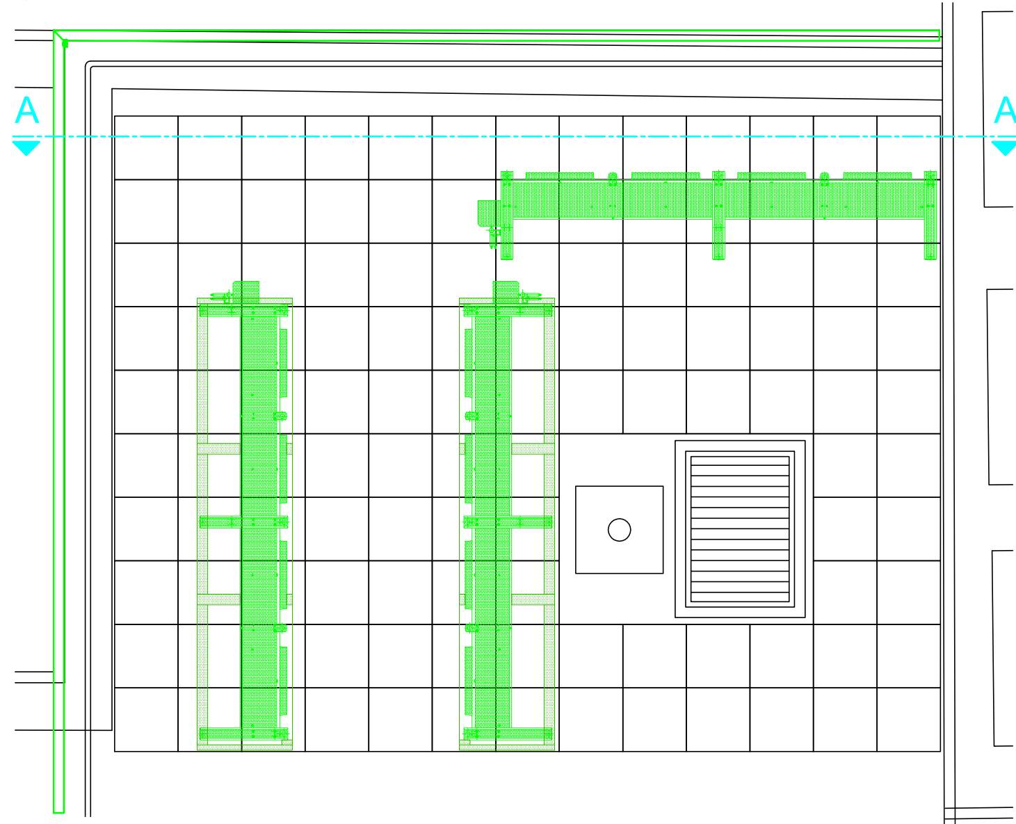
02 Condenser Plan Layout Scale 1:50 @ A3
