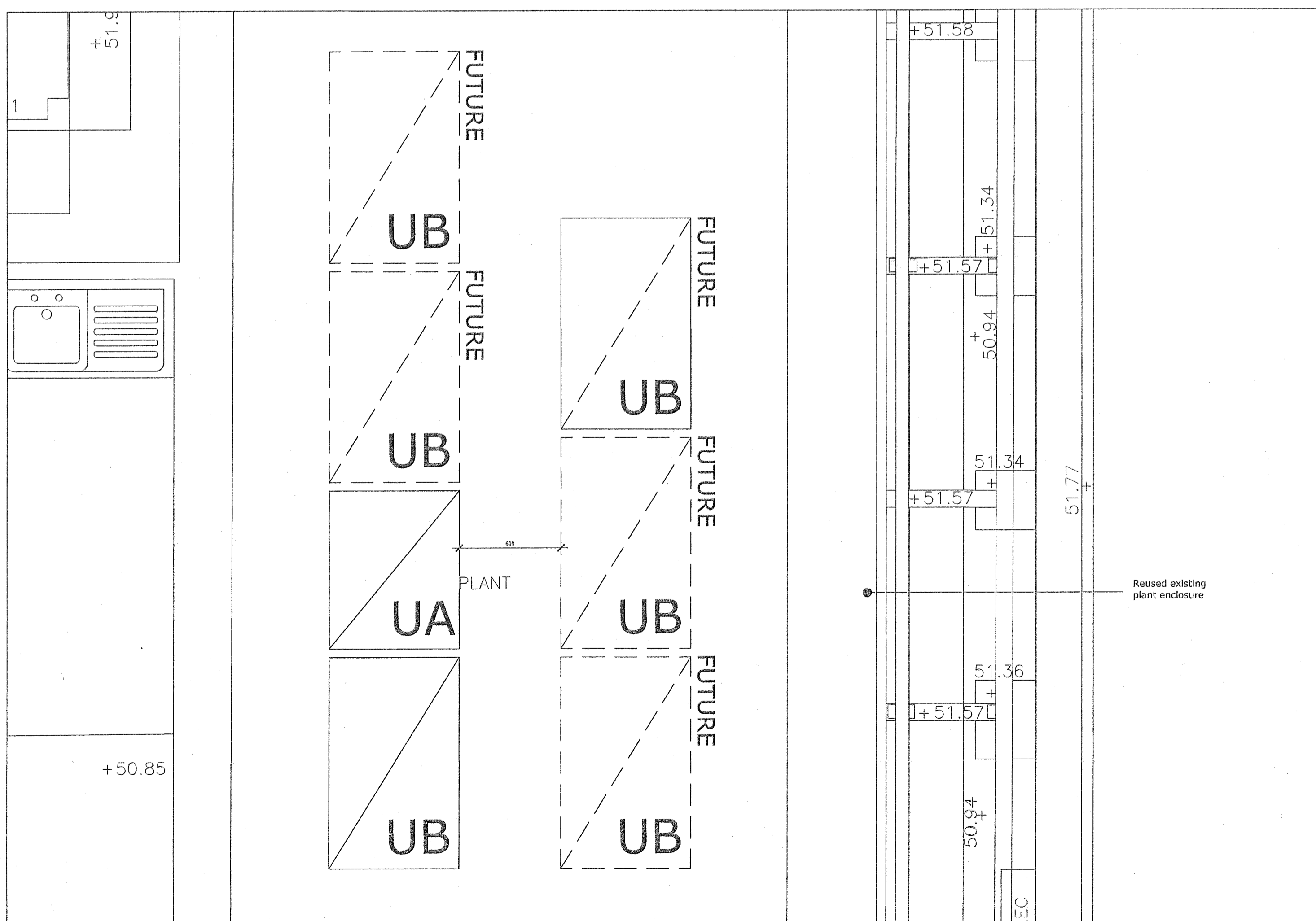
2 Proposed 11th Floor Roof Detail Scale 1:20
