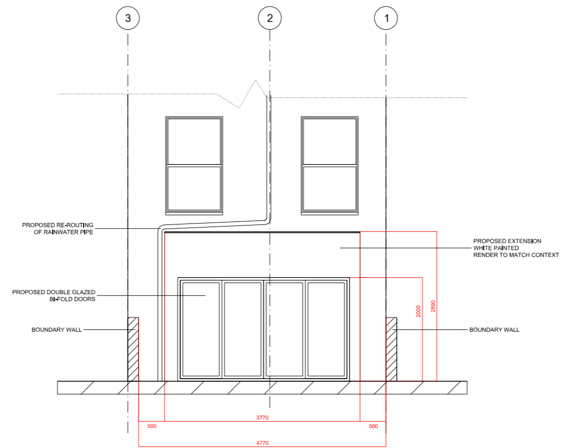
02 PROPOSED BACK ELEVATION
