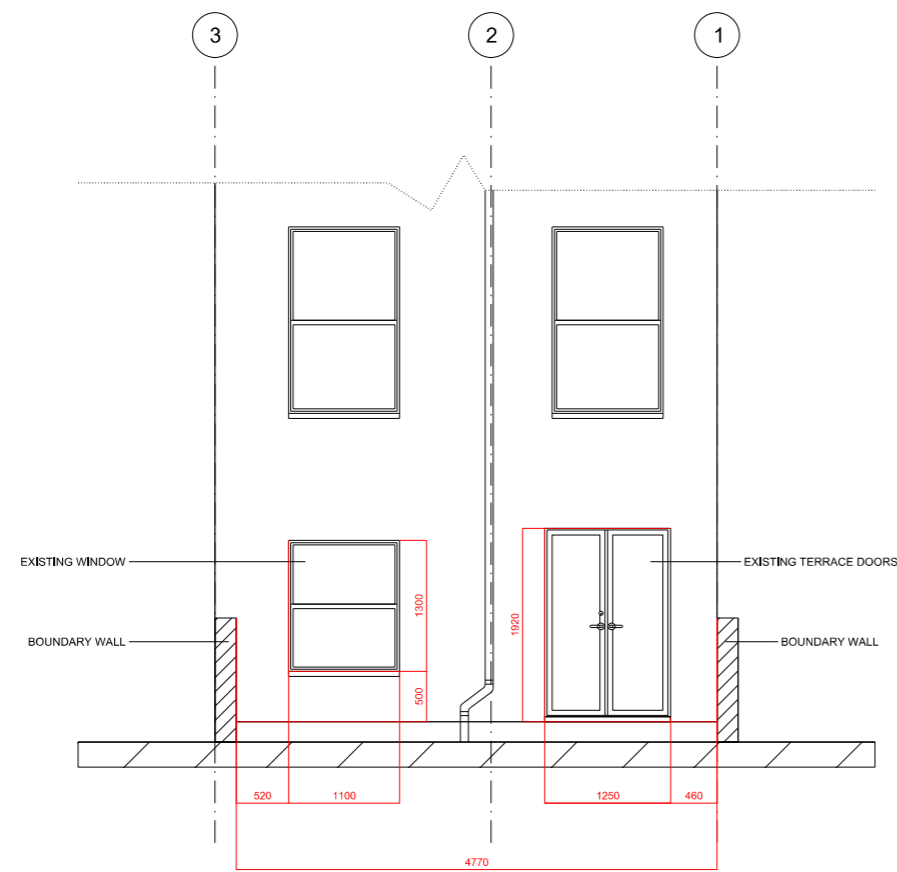
01 EXISTING BACK ELEVATION
