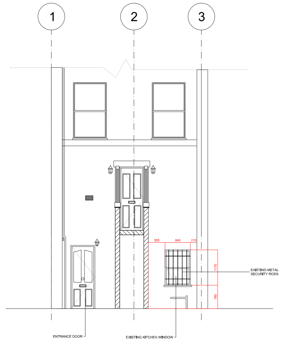
01 EXISTING FRONT ELEVATION
