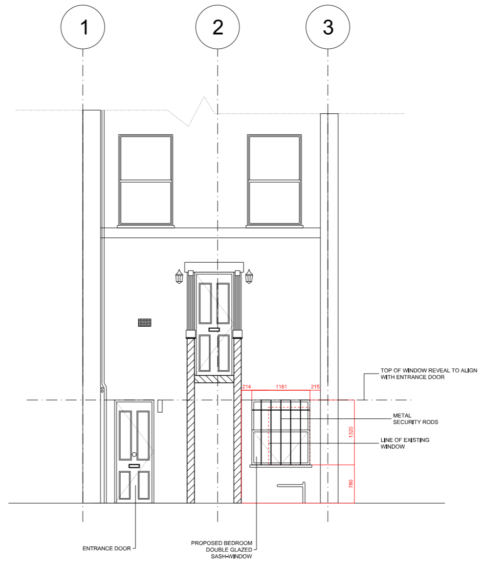
02 PROPOSED FRONT ELEVATION
