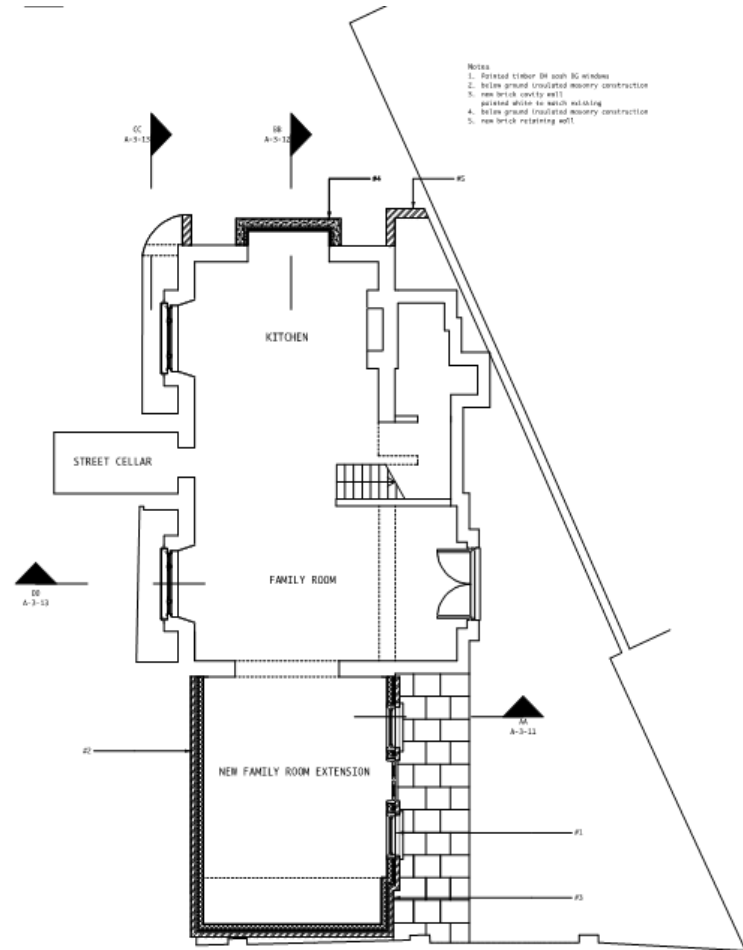
Proposed Lower ground floor
