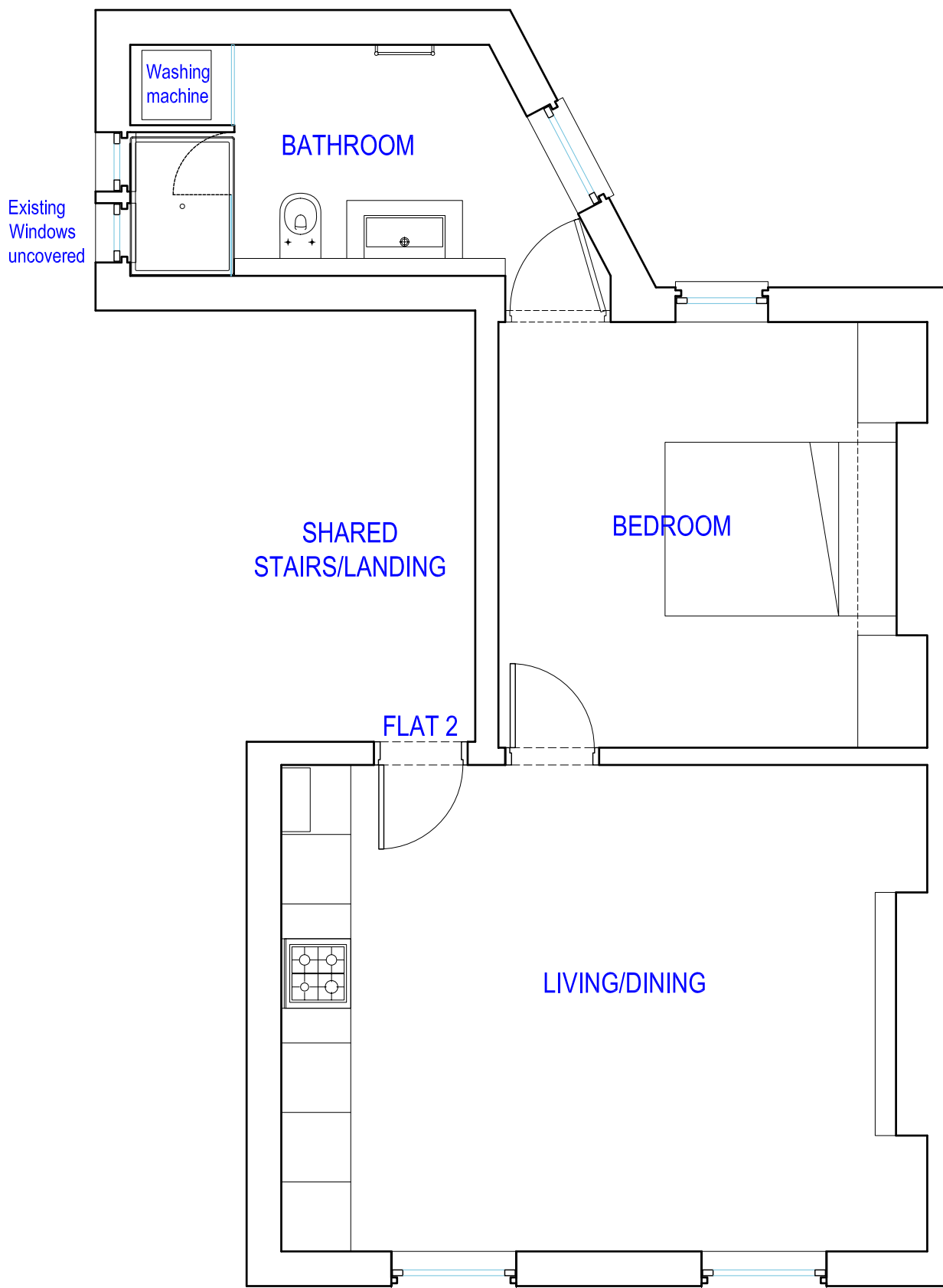
PROPOSED FIRST FLOOR PLAN - 2 CONWAY STREET
