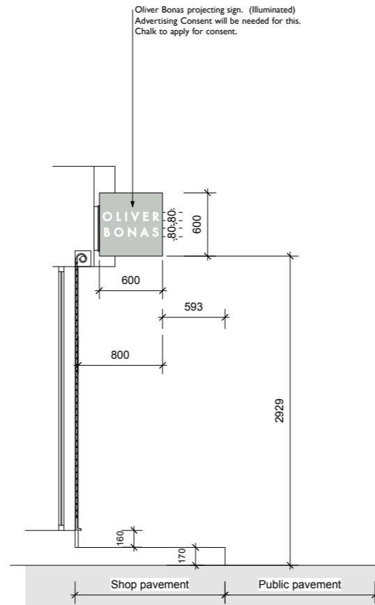
2 Shopfront section
