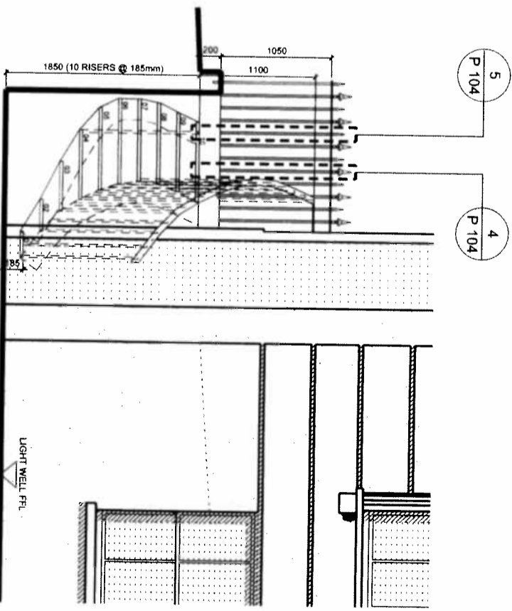
3 DETAIL JOHN ST ELEVATION P 104 1:25
