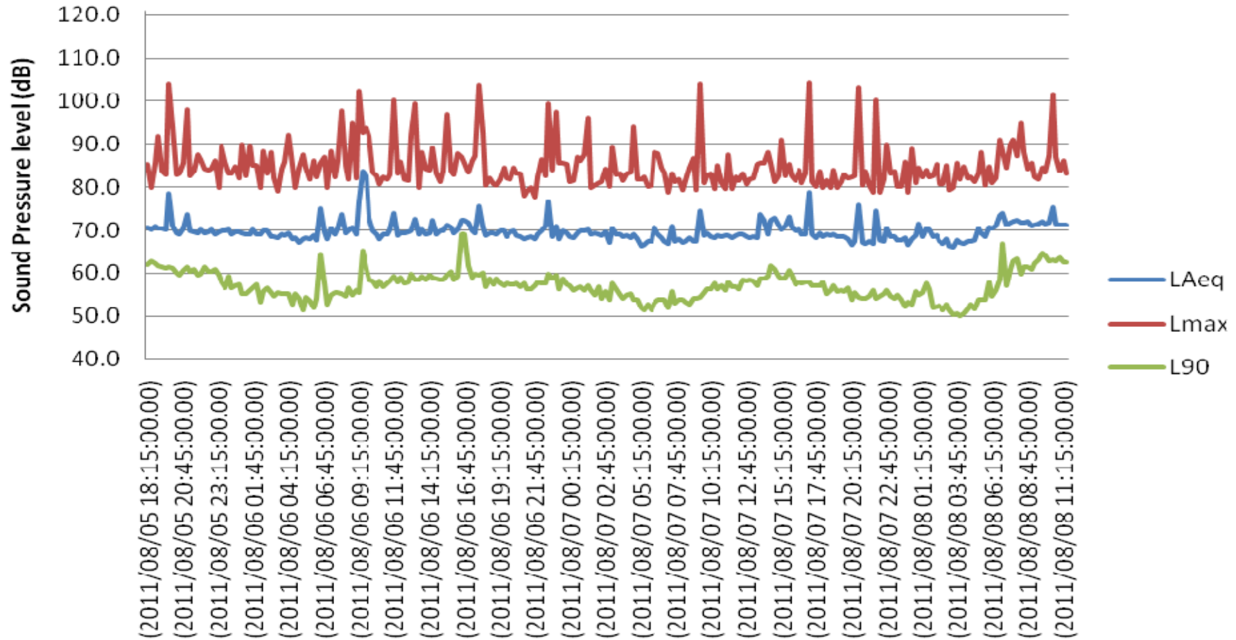
Graph C1: External Noise Time History - Location 1
