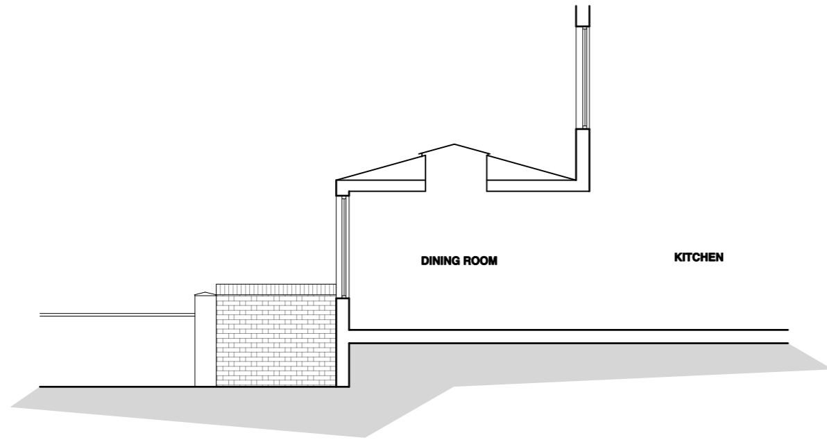
SECTION AA - EXISTING 1:100@A3
