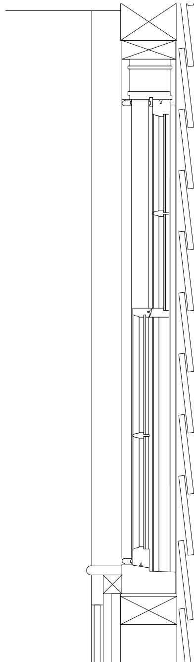
01 Existing window section 1:5@A1, 1:10@A3
