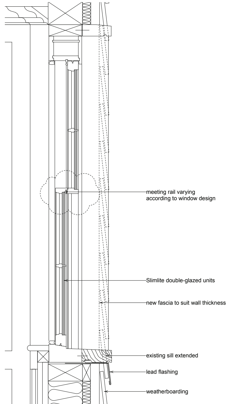
02 Proposed window section 1:5@A1, 1:10@A3
