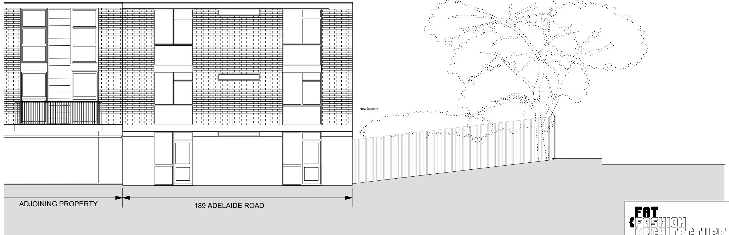
EAST ELEVATION (to access route) AS EXISTING
