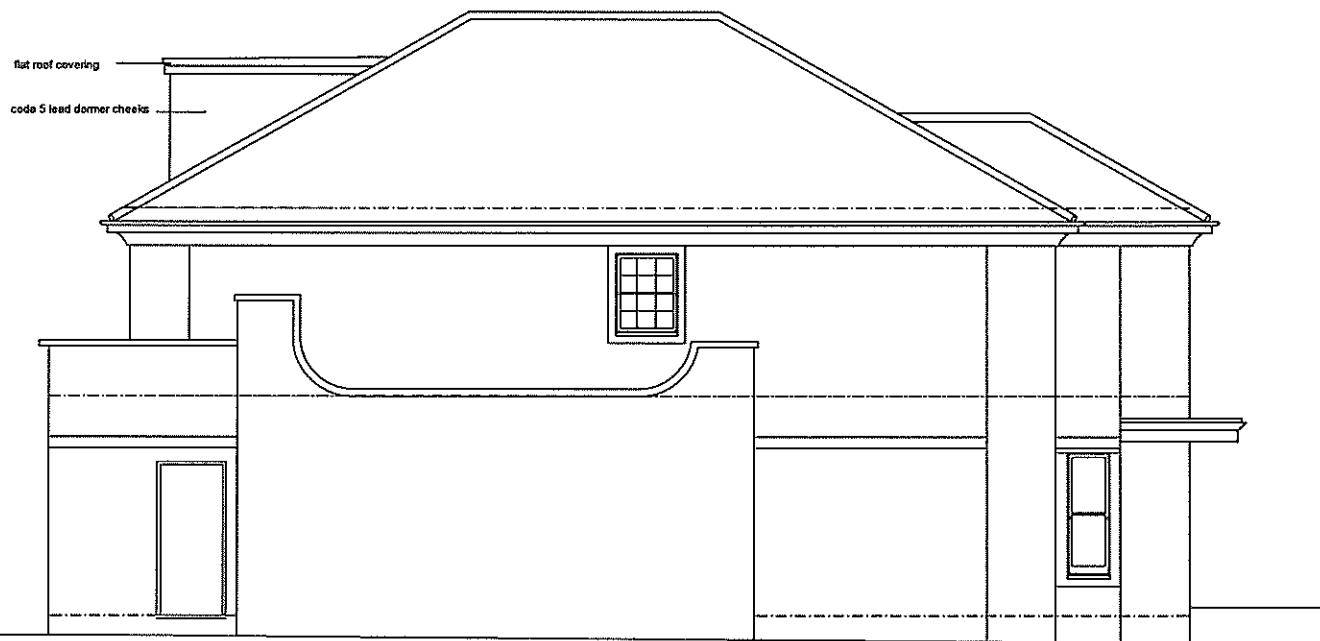
side elevation
