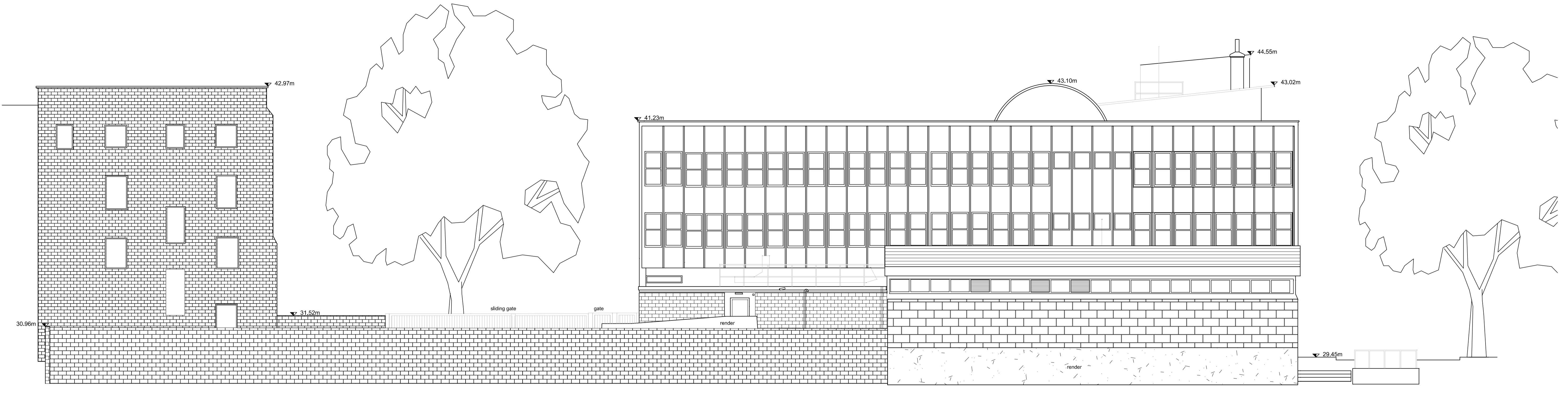
EASTERN ELEVATION
