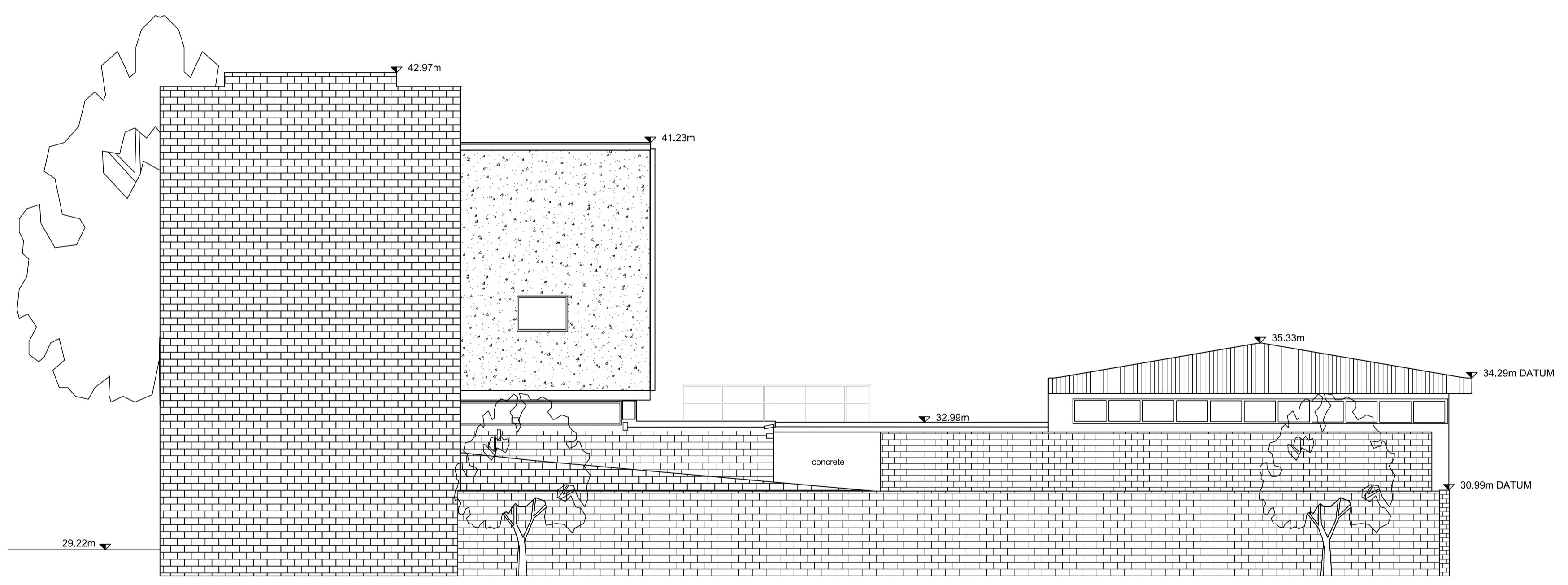
SOUTHERN ELEVATION
