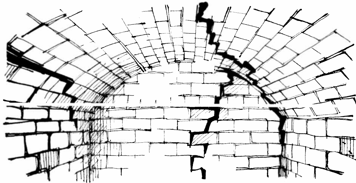
VIEW 1 VAULT 1: CRACKING TO WALLS & ARCH.
