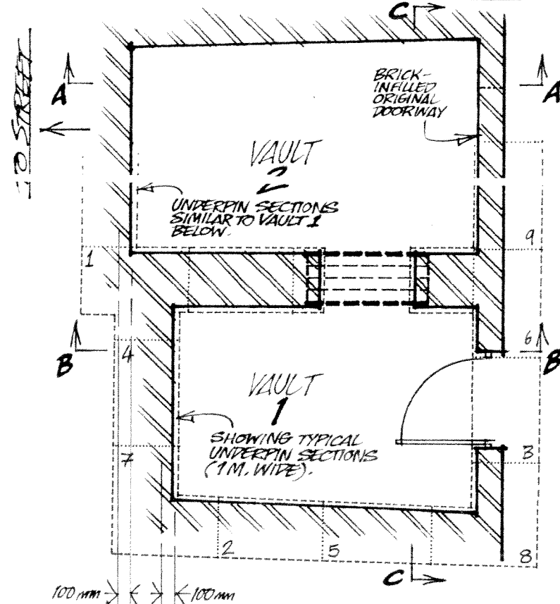
PLAN @ ROOF LEVEL
