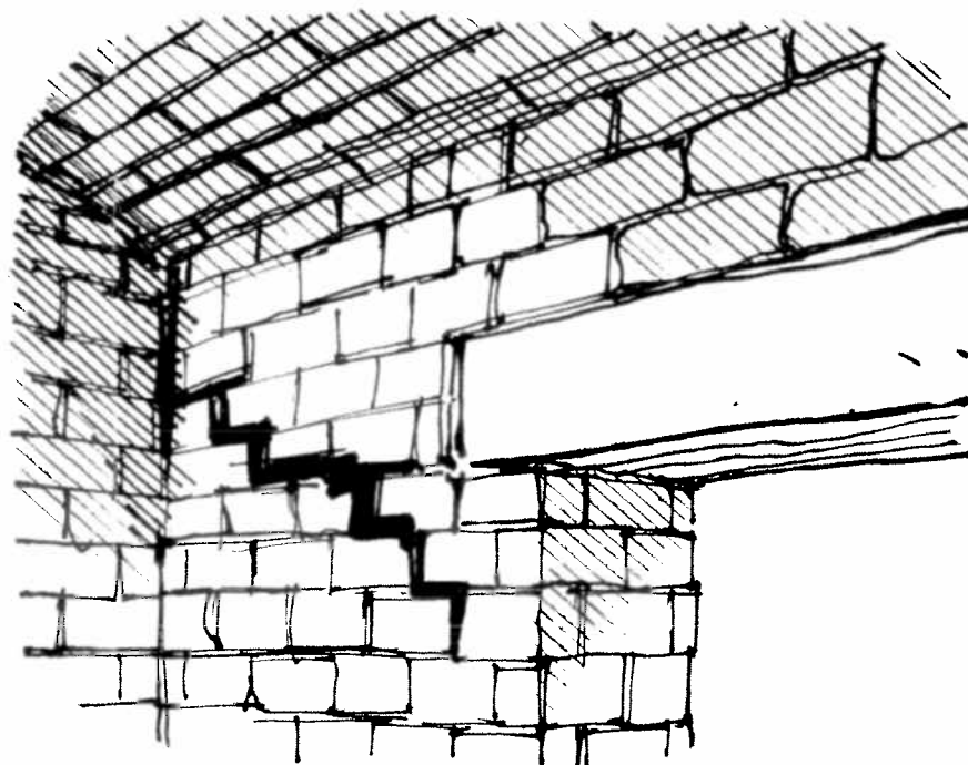
VIEW 4 VAULT 2: CRACKING TO CENTRAL WALL.
