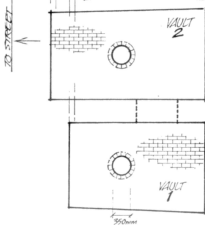
PLAN @ ROOF LEVEL
