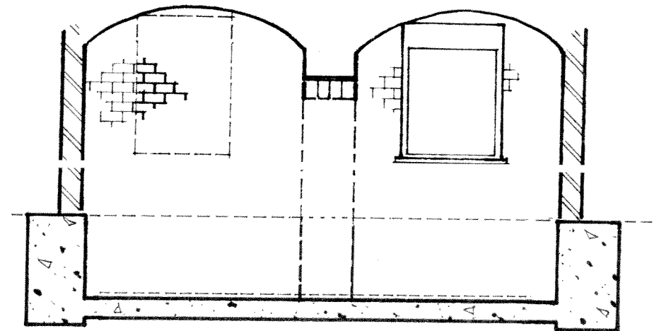
SECTION C-C
