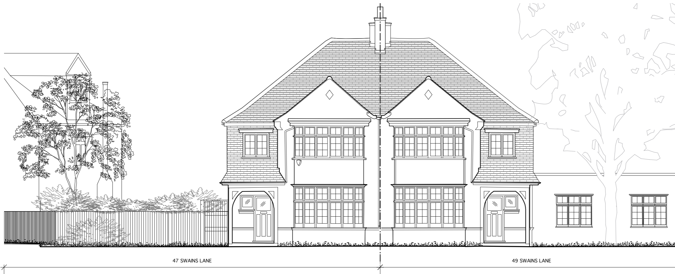
A 010 STREET FRONT ELEVATION
