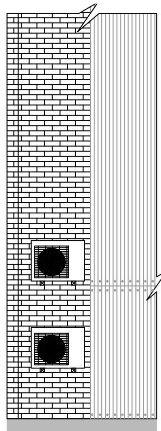
EXISTING ELEVATION B
