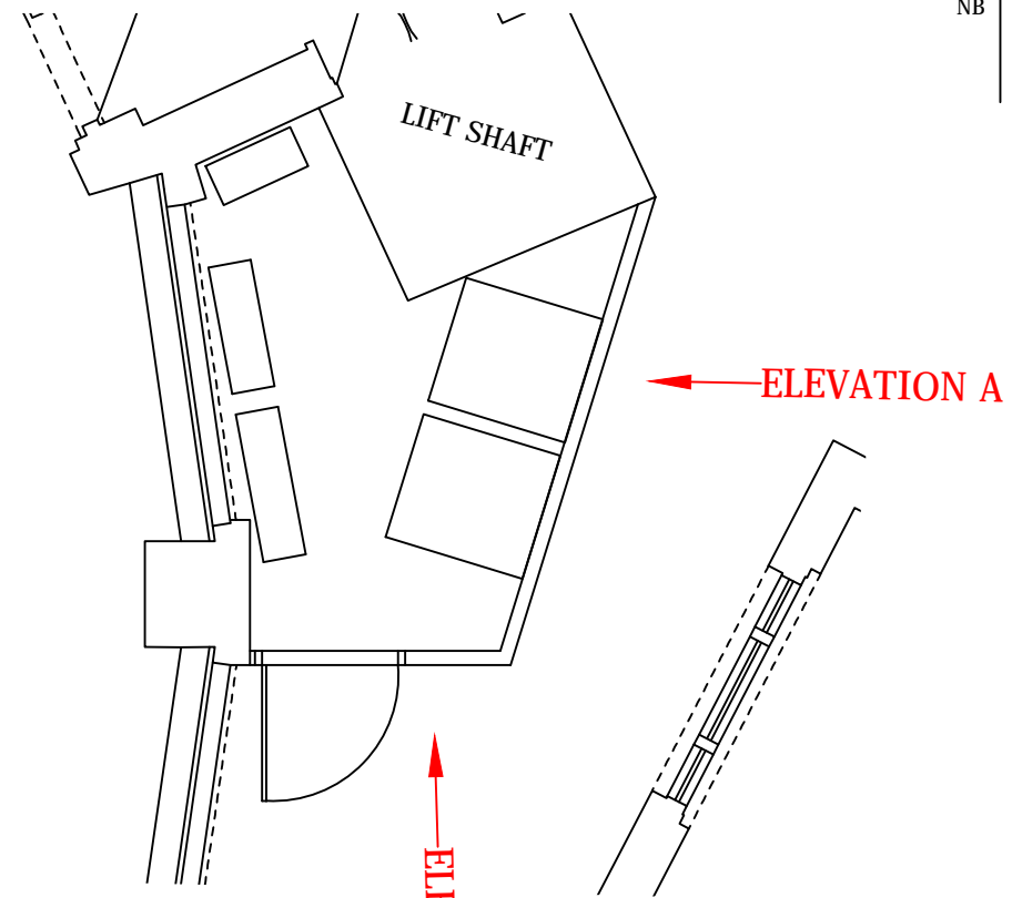
PROPOSED LAYOUT
