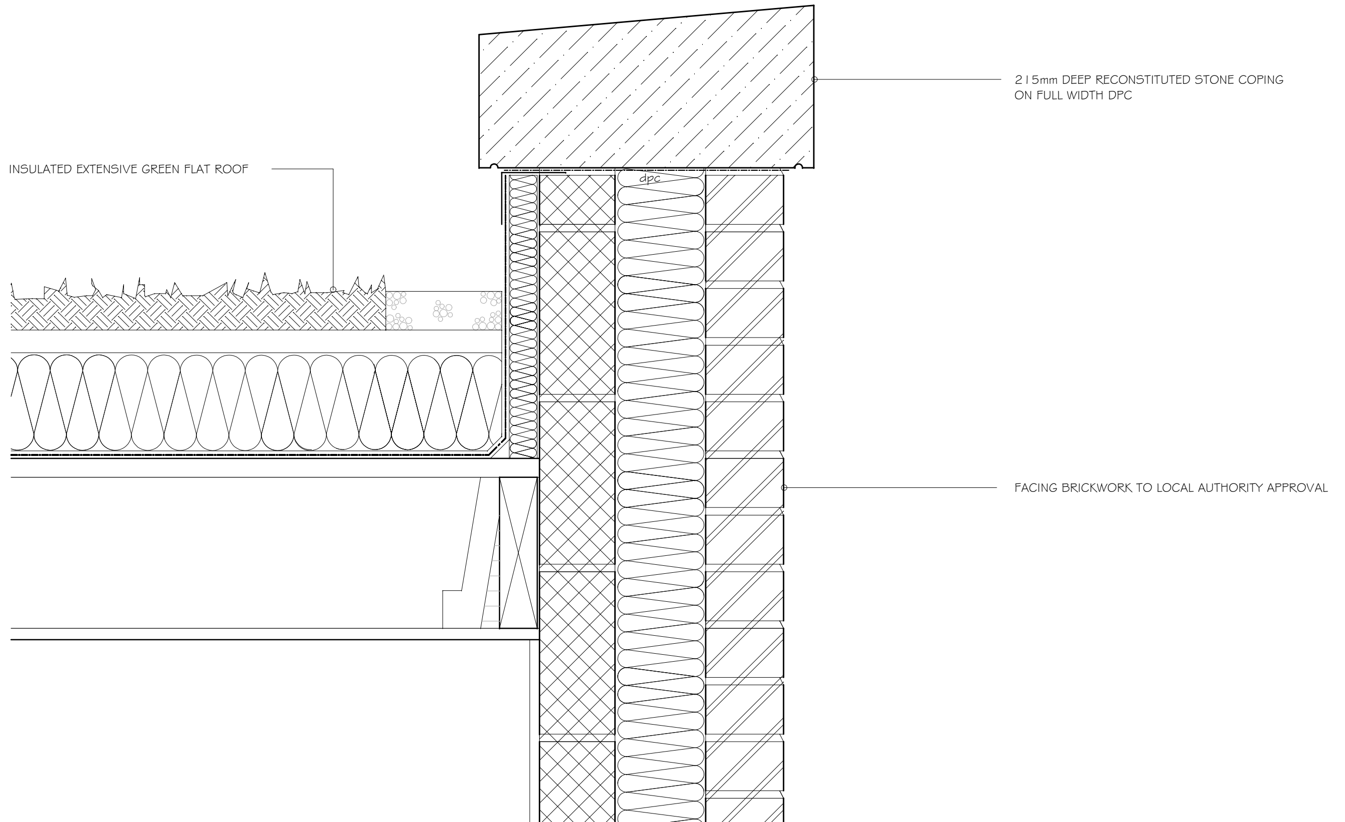
typical flat roof parapet detail
