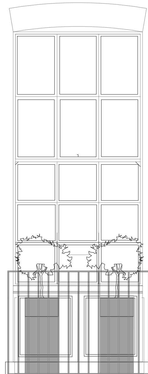
Proposed window elevation with balcony and planters in position
