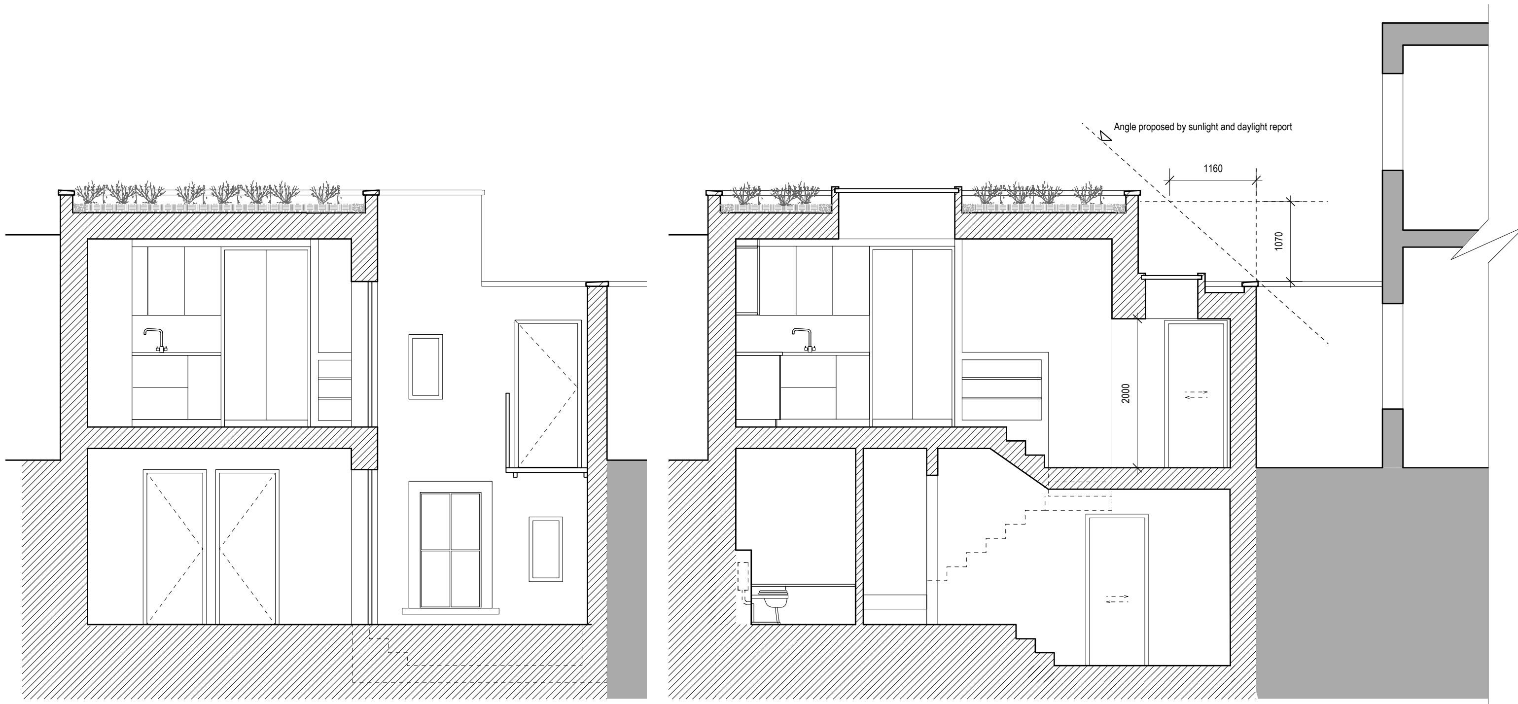
1 Proposed Section 1:50
