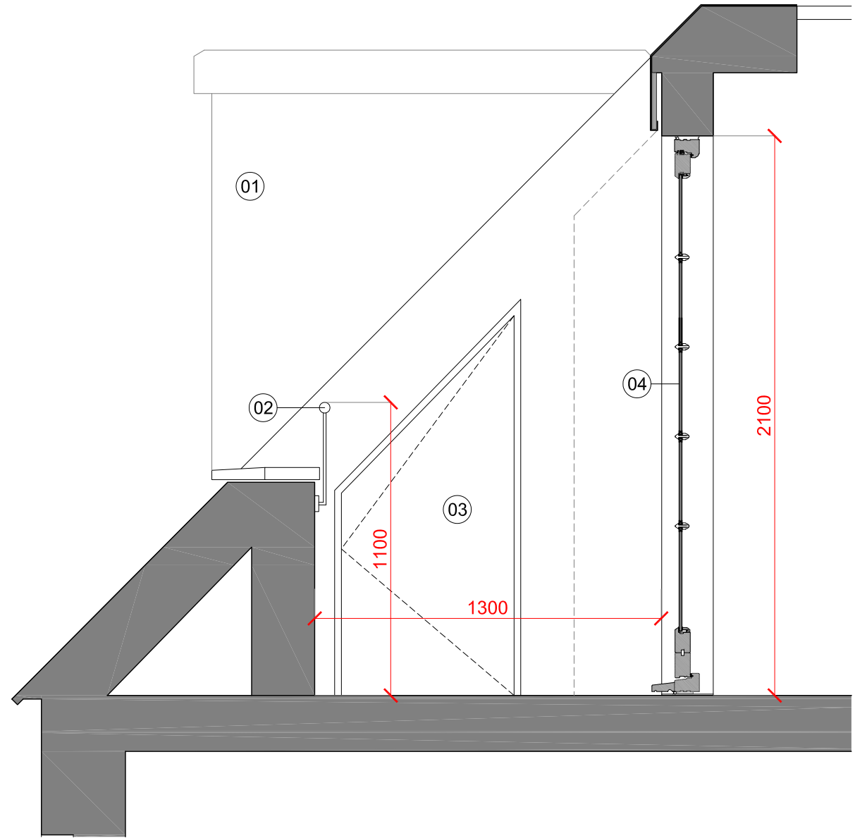
Section - Inset Terrace
