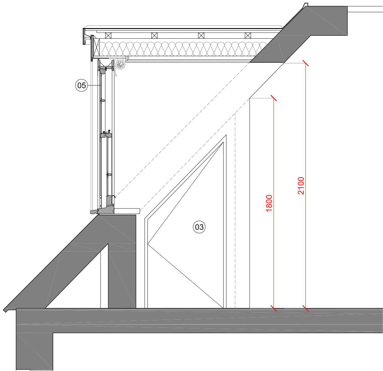
Section - Dormer Window
