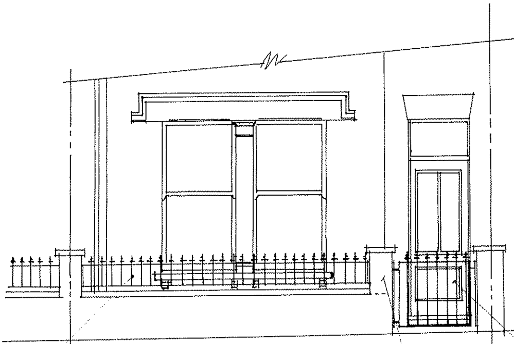
PART FRONT ELEVATION - PROPOSED ALTERATION - railing, pier & gate
