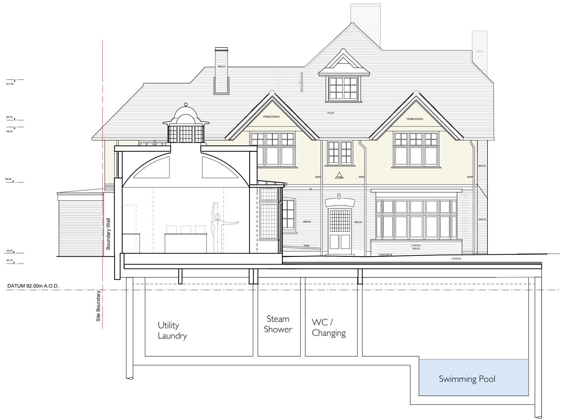
NORTH GARDEN ELEVATION
