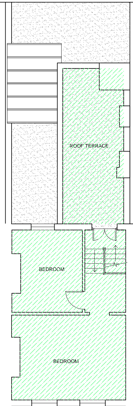
SECOND FLOOR
