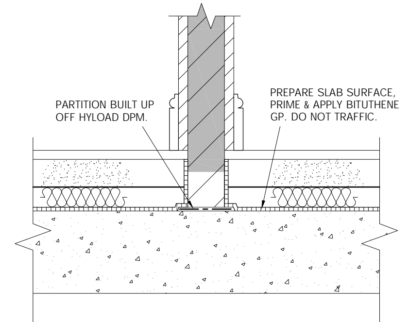
DETAIL E (INTERNAL PARTITION)
