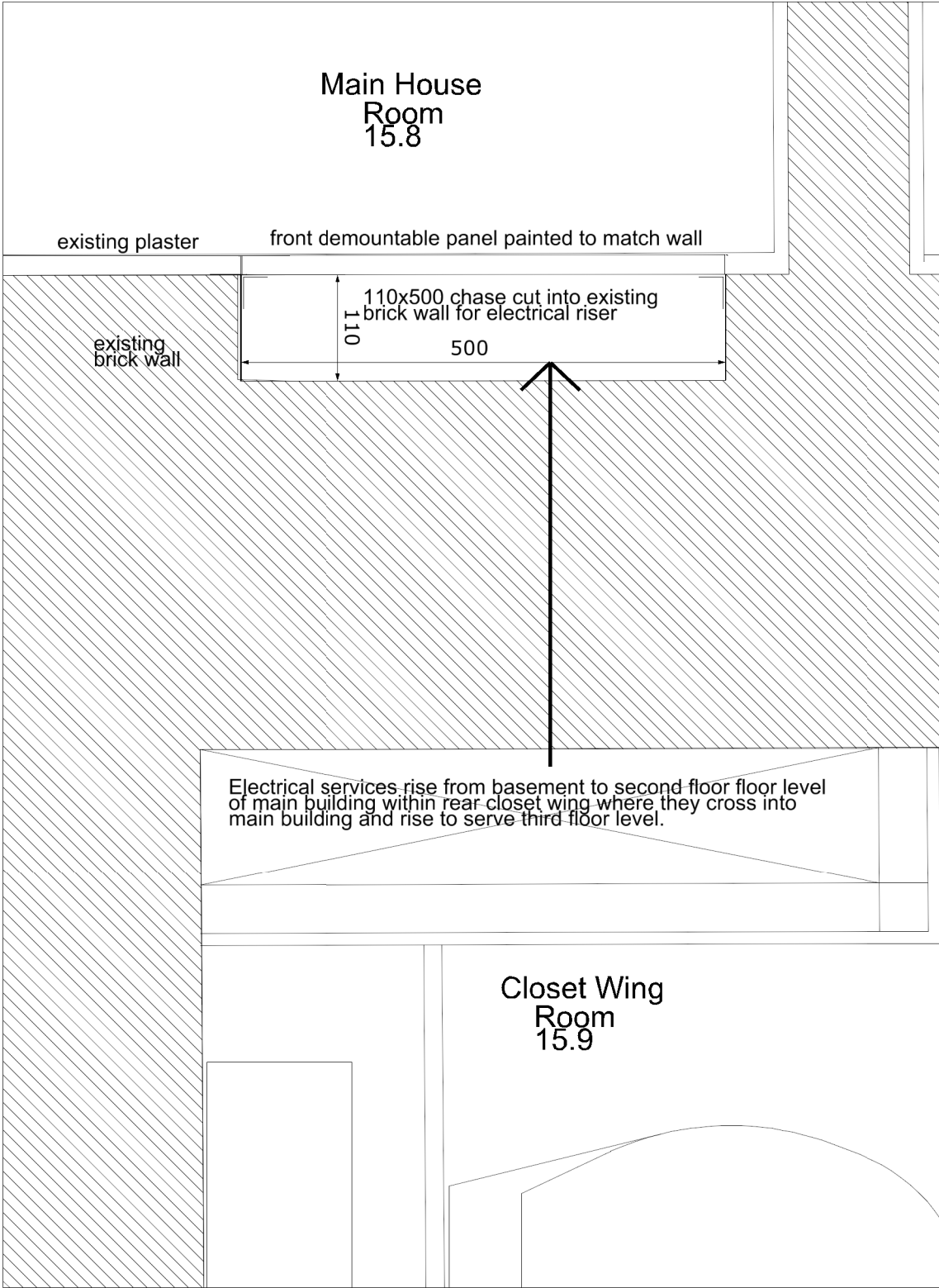
Plan of proposed Electrical Riser at Second Floor Level
