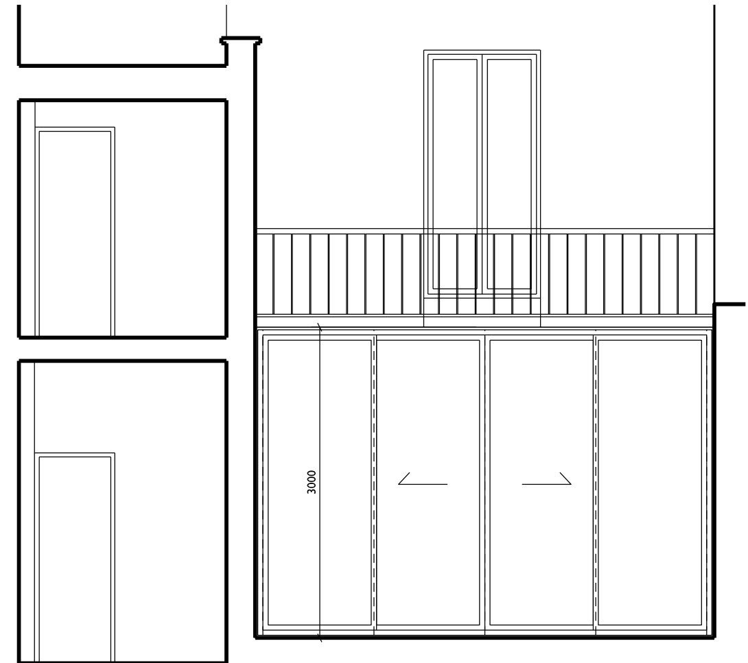
Rear Elevation
