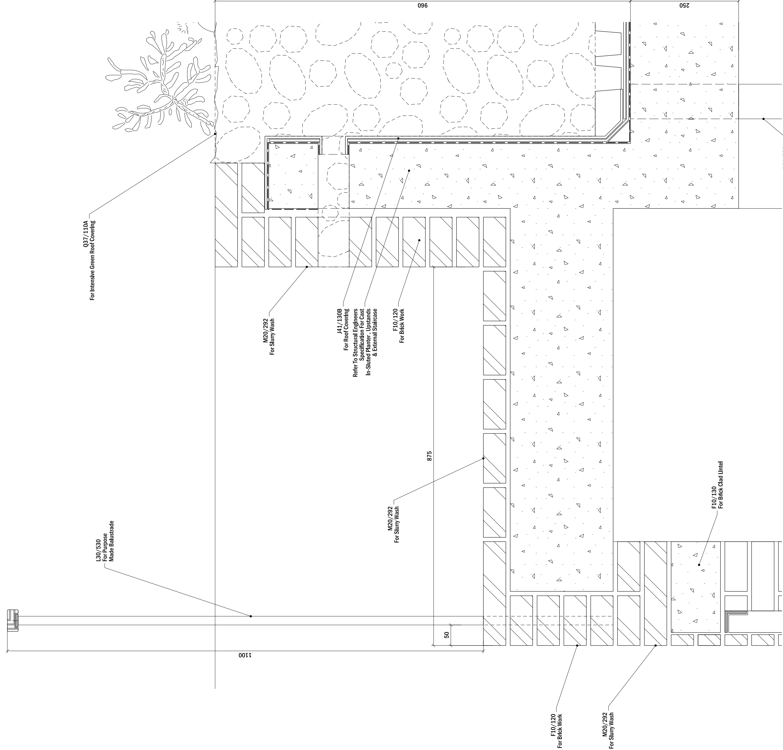
02 Bike Store Head Detail 1:500A1 & 1:100A3
