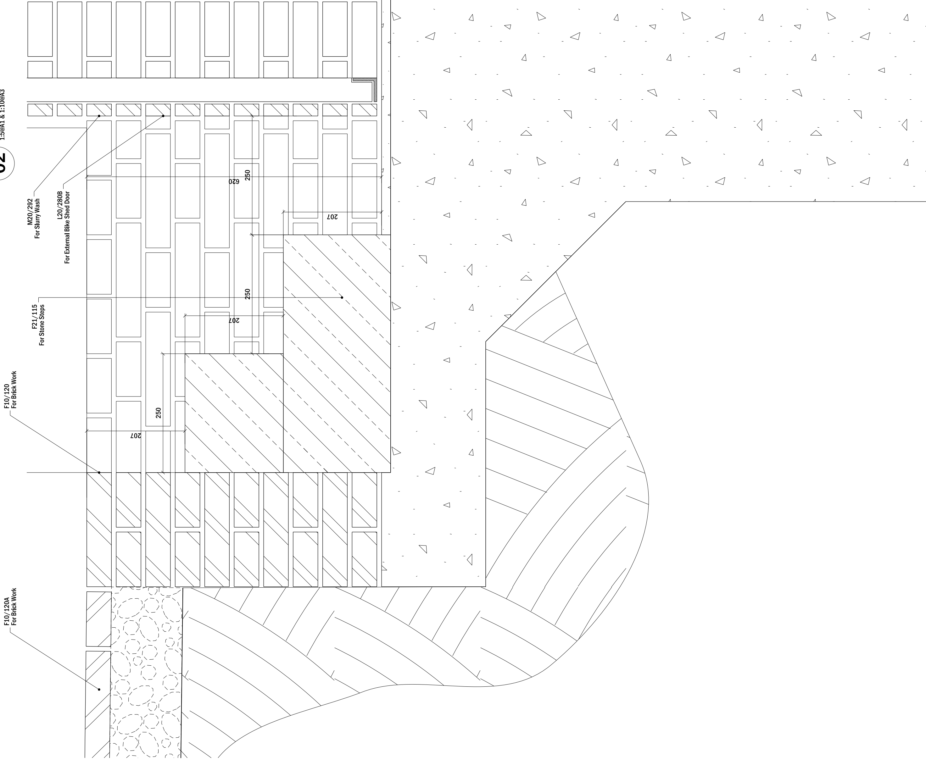
01 Steps To Bike Shed Detail 1:500A1 & 1:100A3
