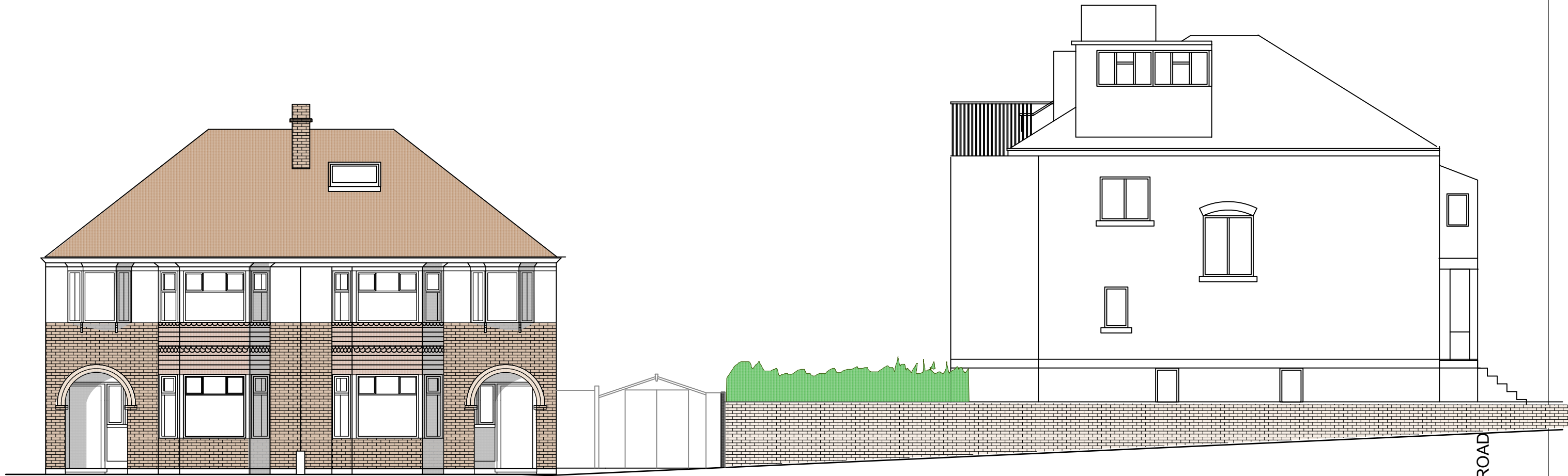
South Elevation
