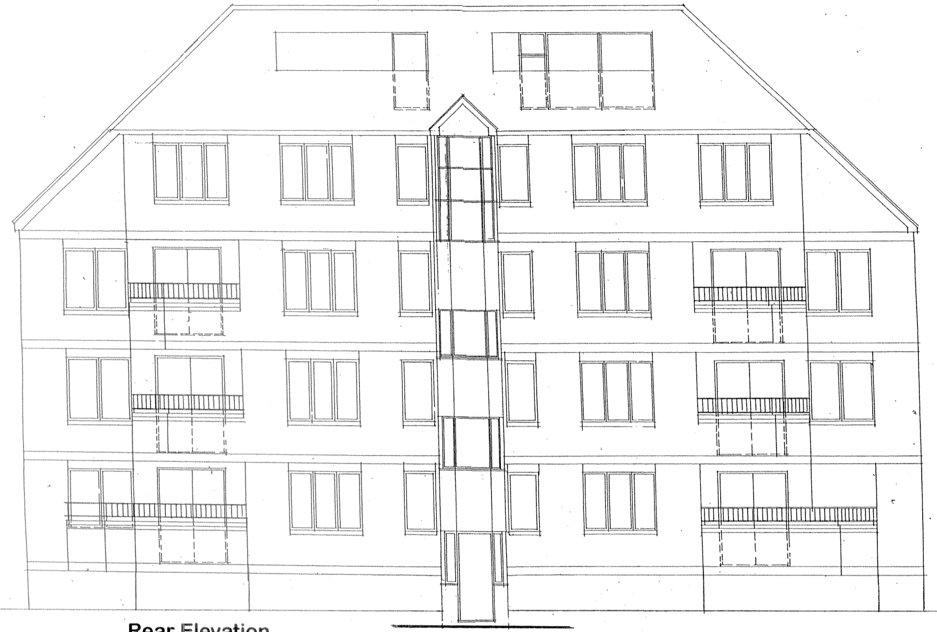
Rear Elevation
