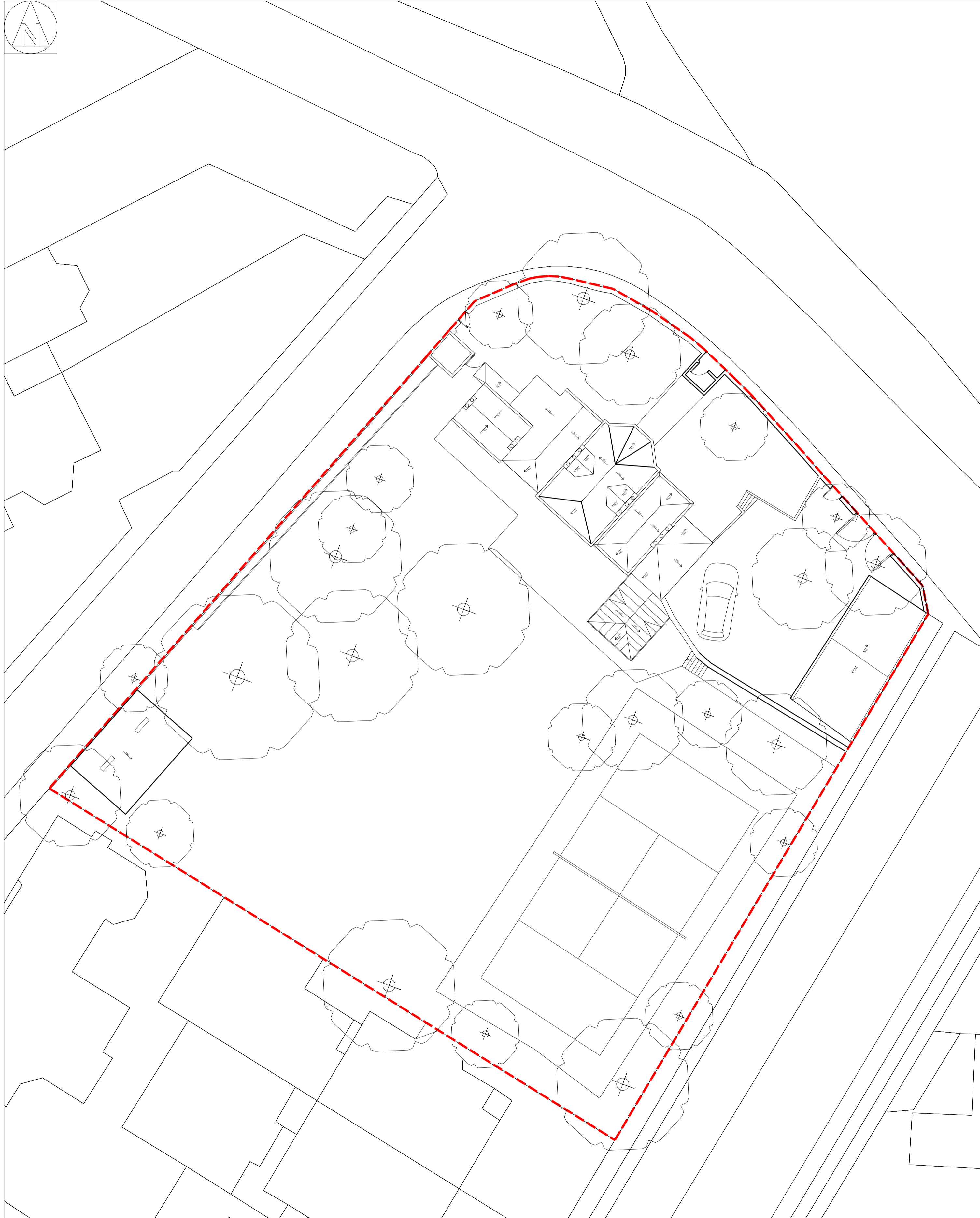
EXISTING SITE PLAN SCALE - 1:200@A1
