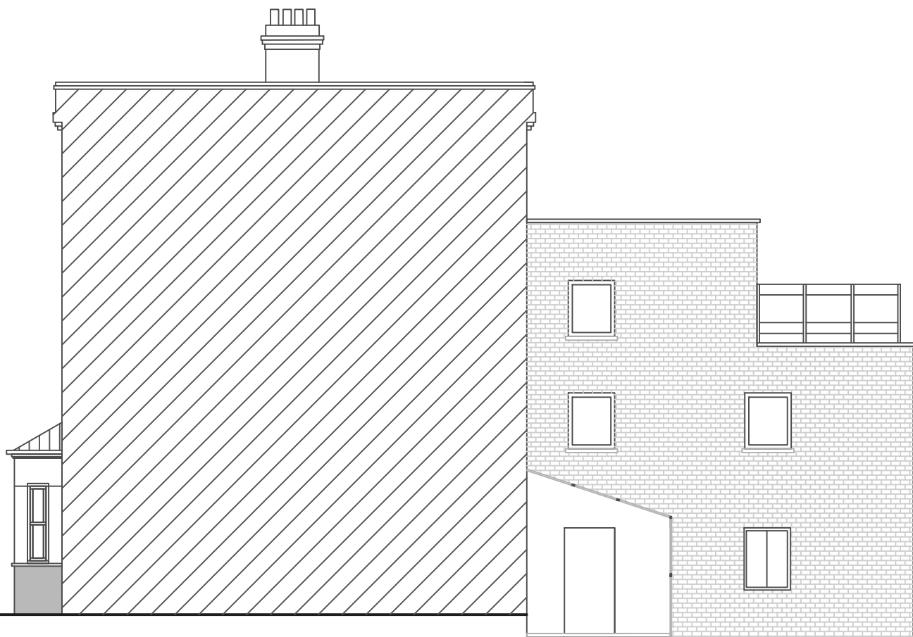
SIDE ELEVATION
