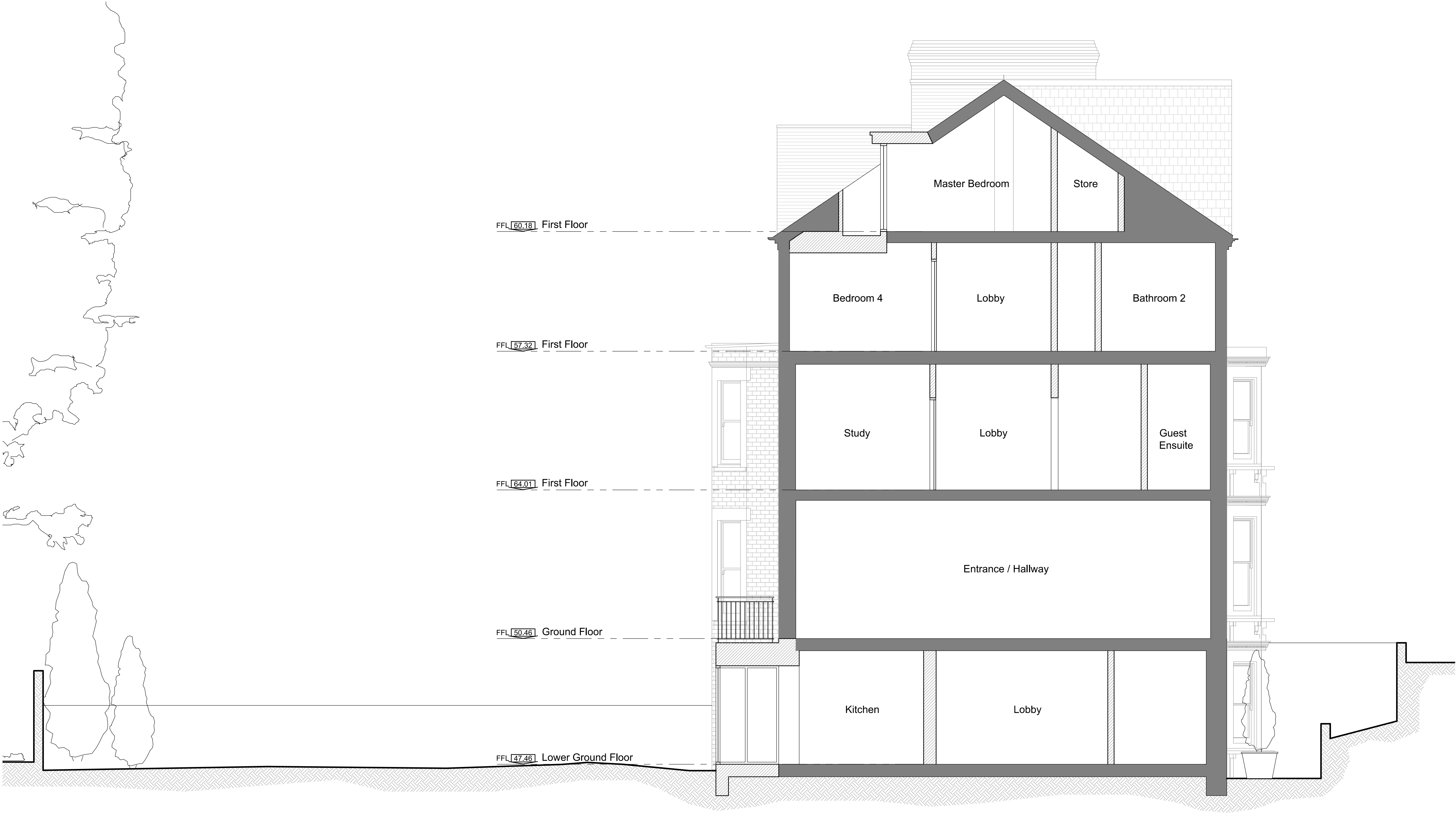
A Approved Section A-A
